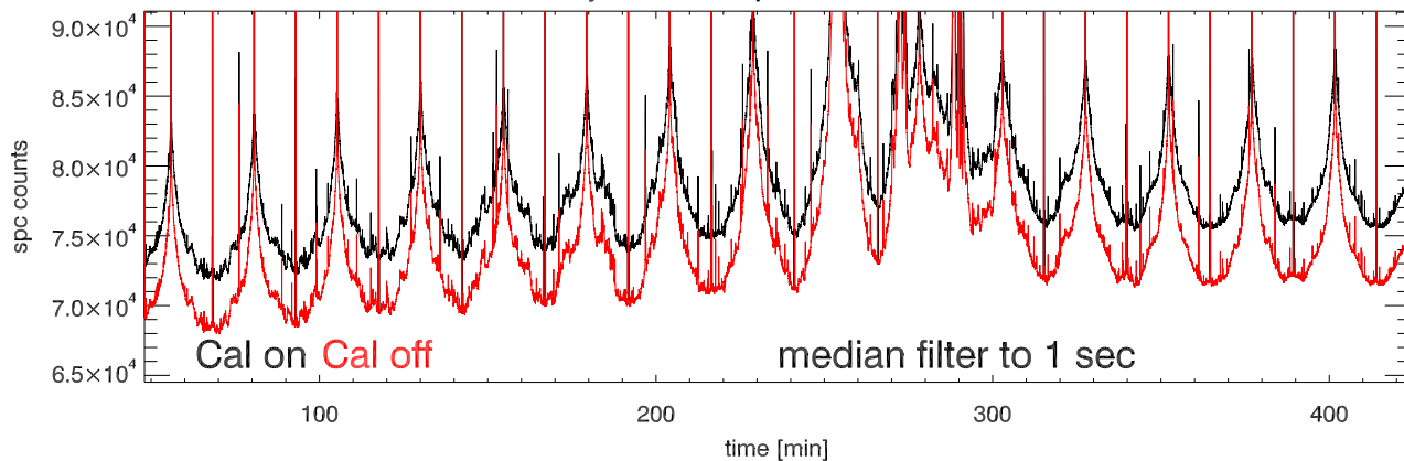
07jul11 a2030 tp vs time. Beam3A
