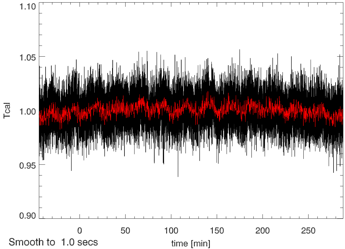
30apr11 calOn - calOff Beam2A SigA: 0.027
