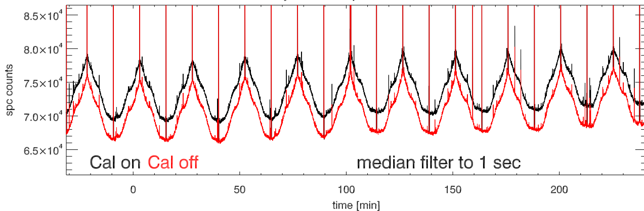
23may11 a2030 tp vs time. Beam2A
