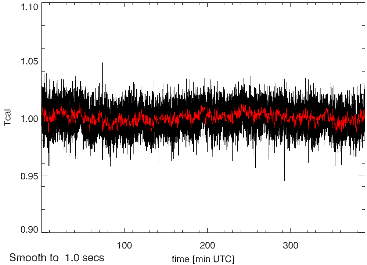
11mar13 calOn - calOff Beam2A SigA: 0.018
