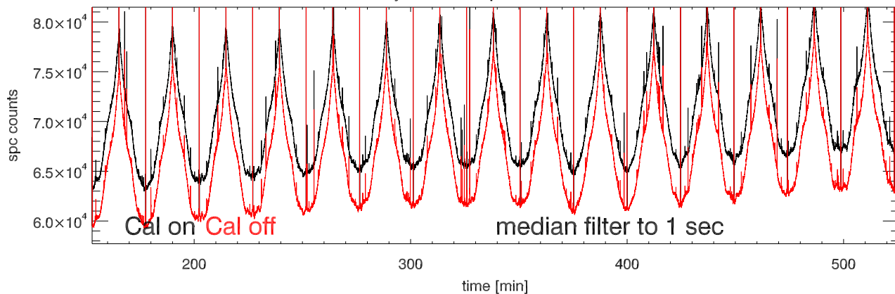
03may12 a2030 tp vs time. Beam2A
