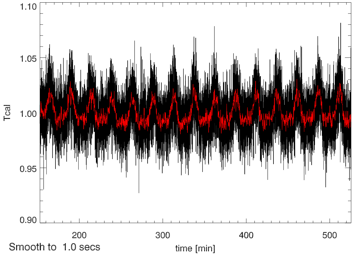
03may12 calOn - calOff Beam2A SigA: 0.029
