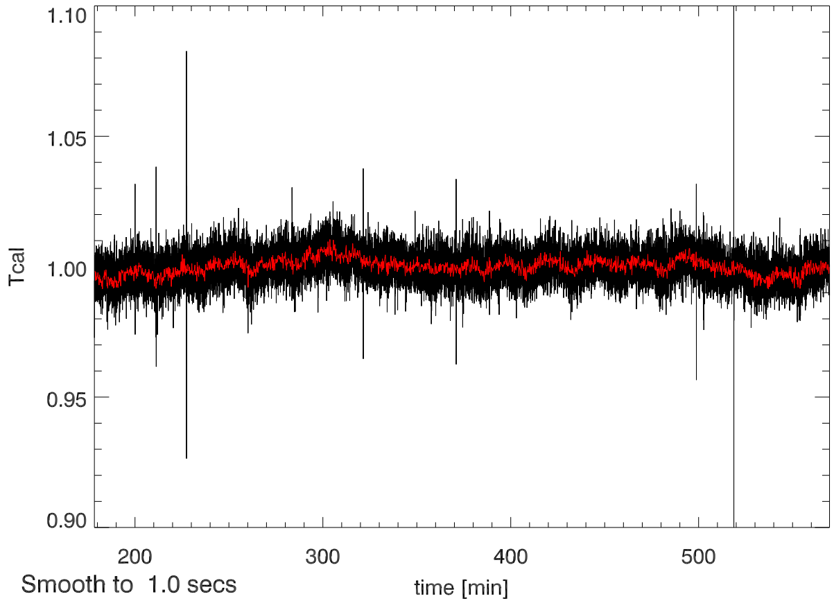
26jul12 calOn - calOff Beam1A SigA: 0.010
