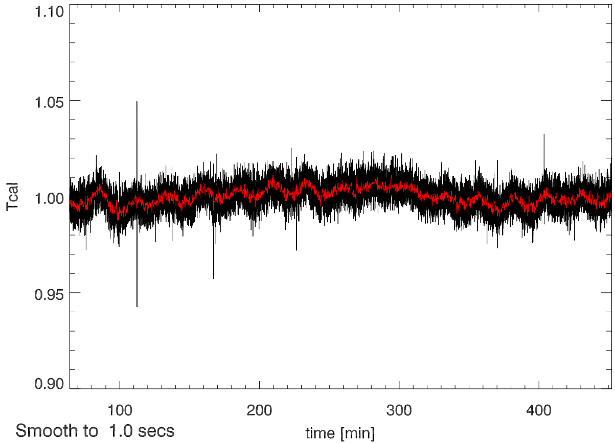
25feb13 calOn - calOff Beam1A SigA: 0.010
