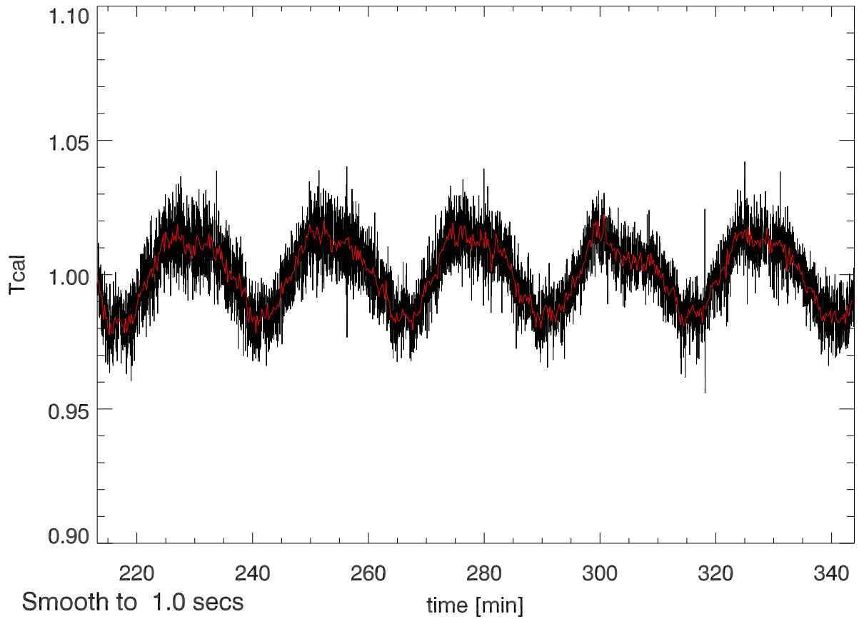
23oct11 calOn - calOff Beam1A SigA: 0.017
