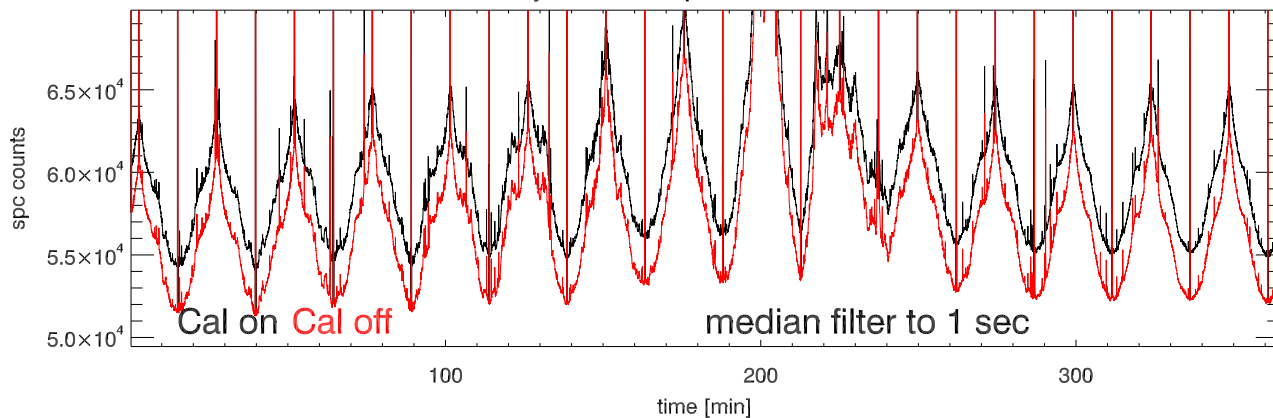
22jul11 a2030 tp vs time. Beam1A
