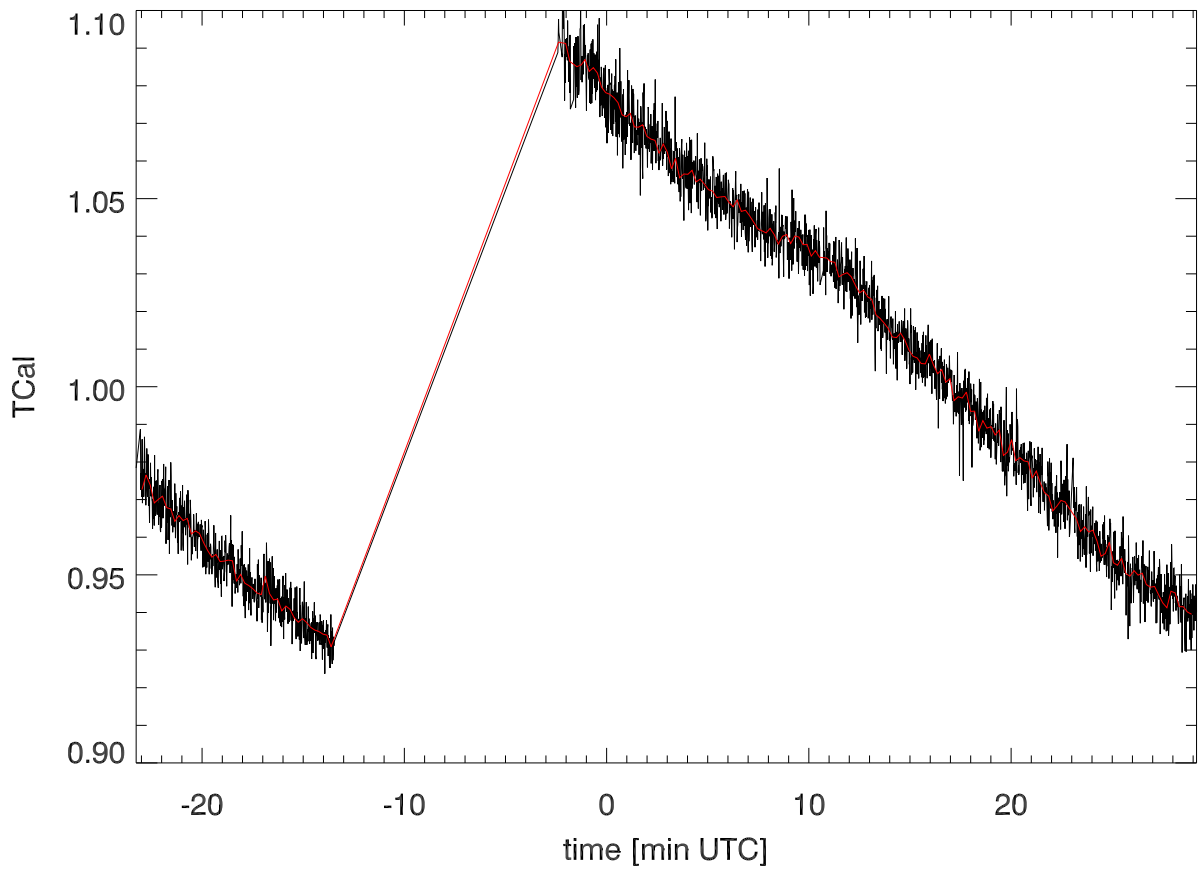
calOn - calOff Beam1B SigB: 0.048
