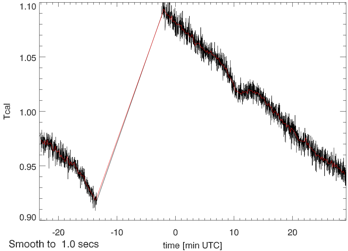
21jan16 calOn - calOff Beam1A SigA: 0.049
