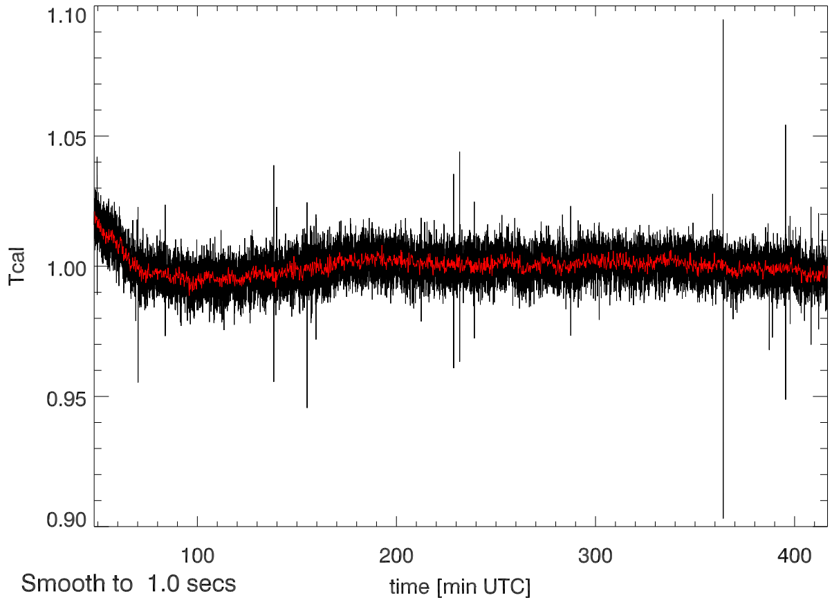
21aug13 calOn - calOff Beam1A SigA: 0.010
