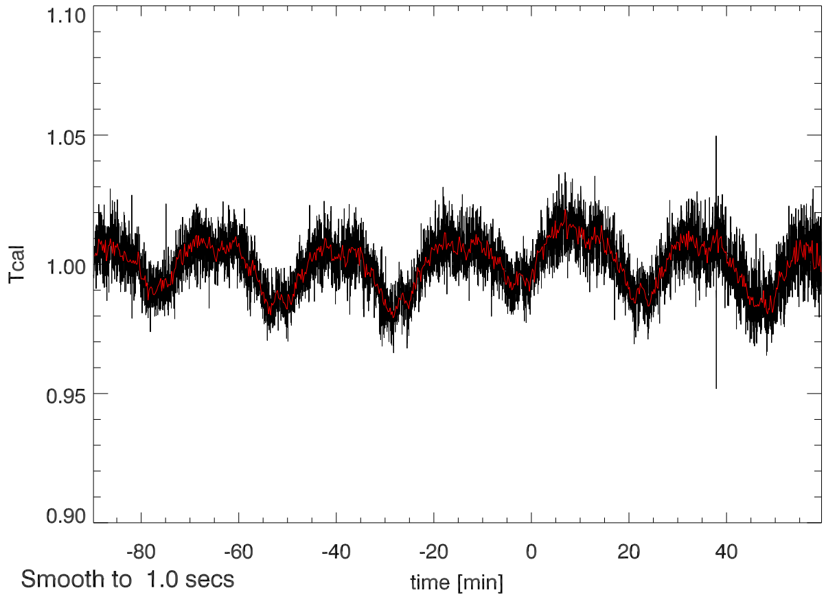
13nov11 calOn - calOff Beam1A SigA: 0.015
