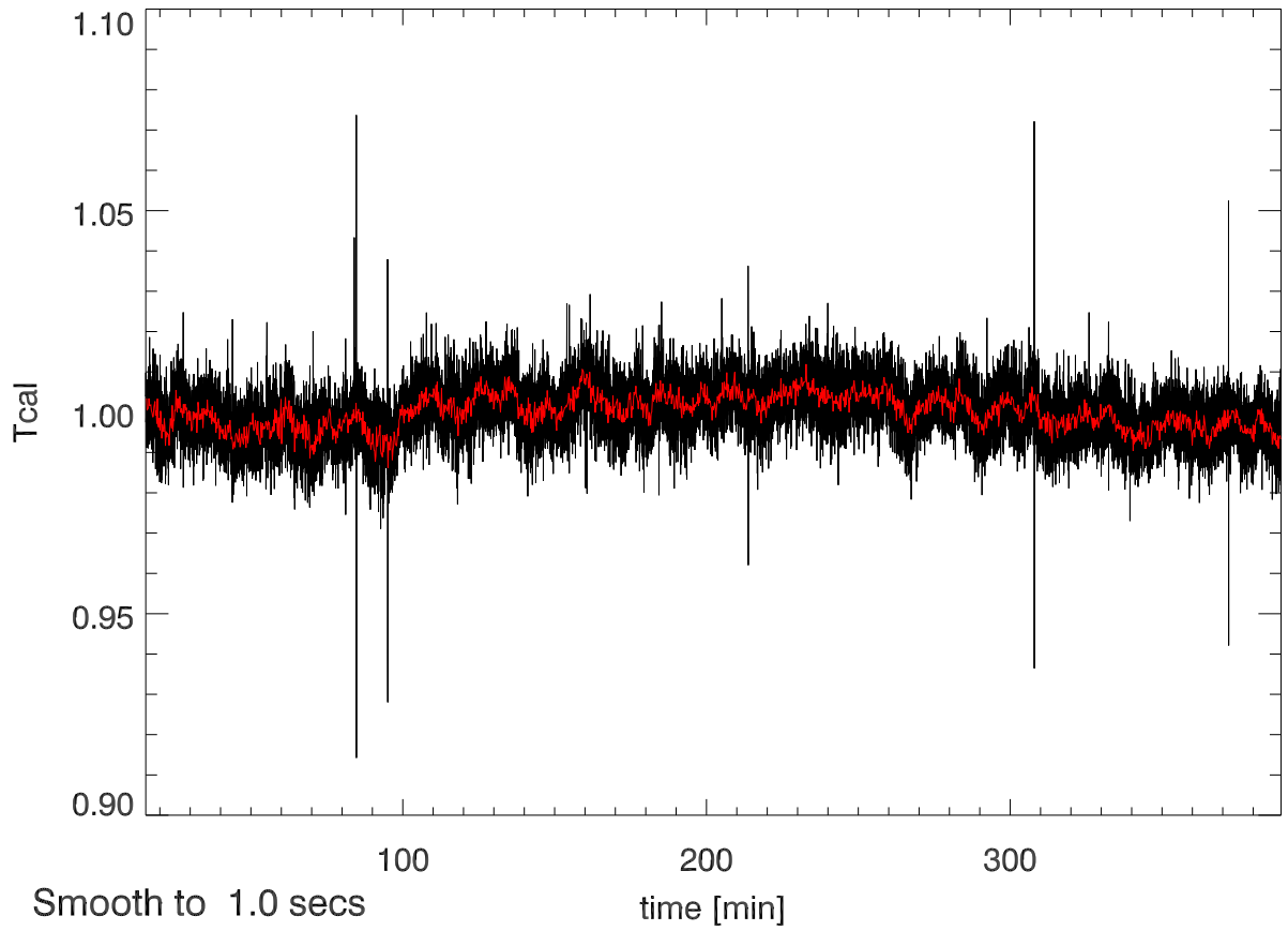
09sep12 calOn - calOff Beam1A SigA: 0.011
