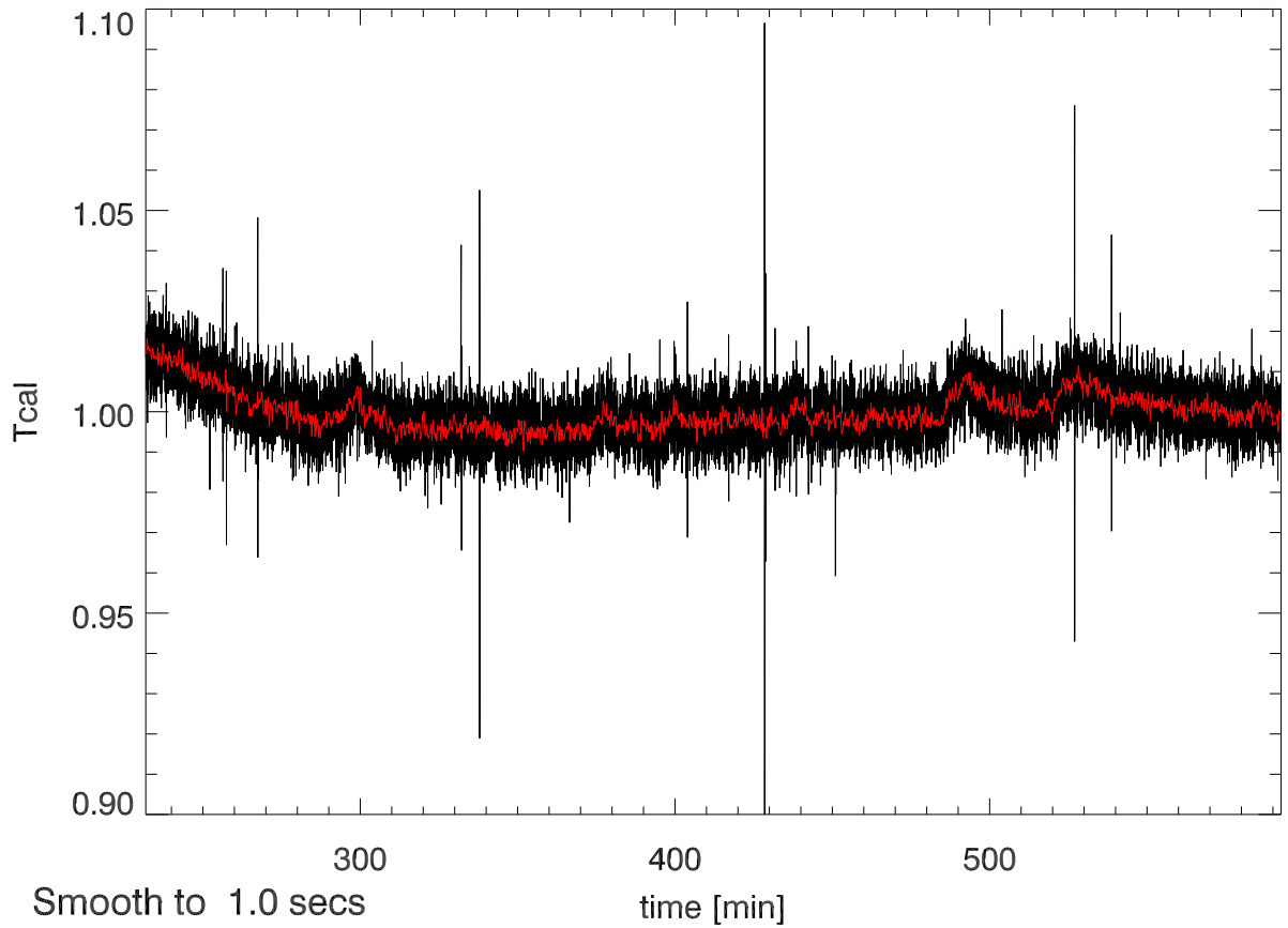
03jan13 calOn - calOff Beam1A SigA: 0.010
