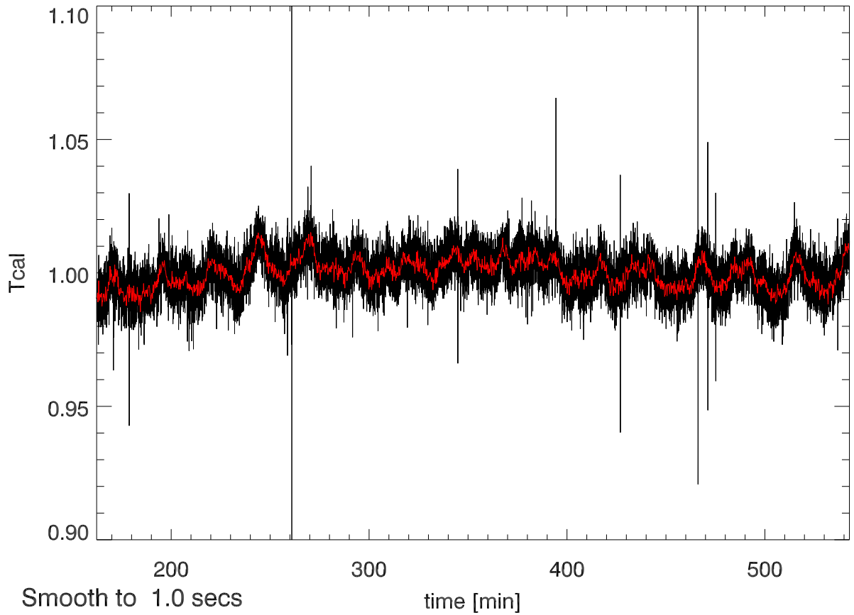
02feb13 calOn - calOff Beam1A SigA: 0.011
