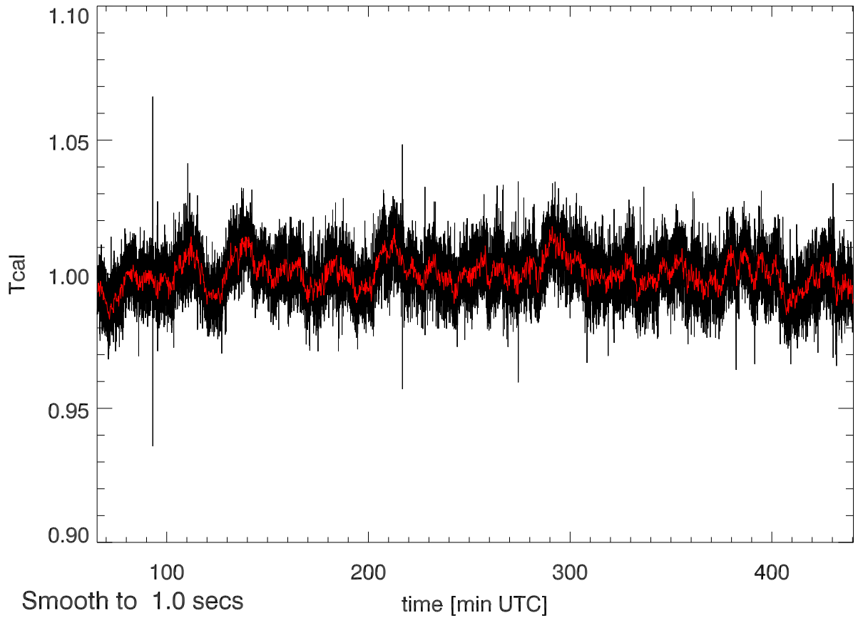
28feb13 calOn - calOff Beam0A SigA: 0.014
