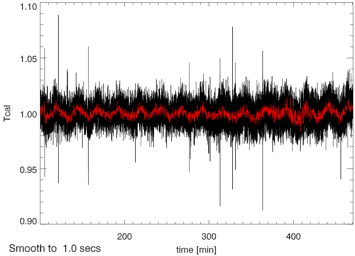
25jun11 calOn - calOff Beam0A SigA: 0.017
