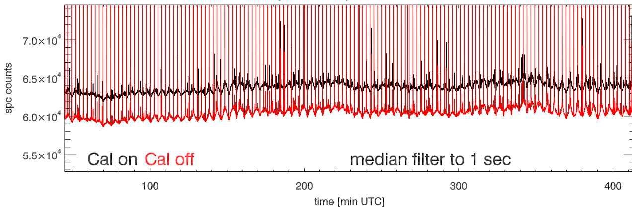
21may13 a2030 tp vs time. Beam0A
