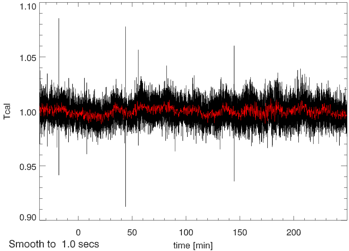
21may11 calOn - calOff Beam0A SigA: 0.016
