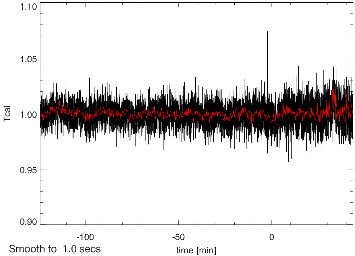
18nov11 calOn - calOff Beam0A SigA: 0.018
