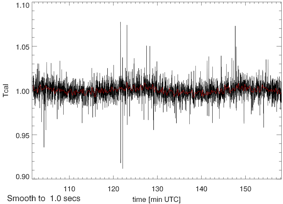
18dec15 calOn - calOff Beam0A SigA: 0.015
