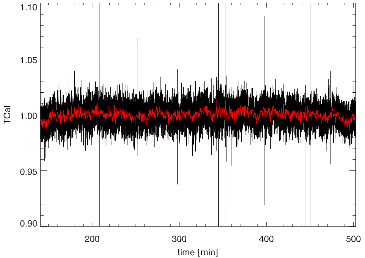
calOn - calOff Beam0B SigB: 0.017
