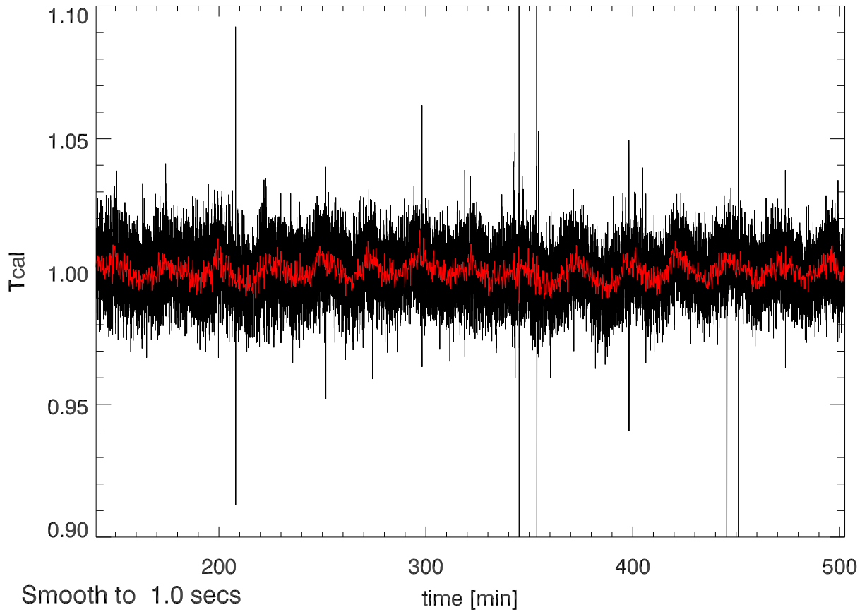
17jun11 calOn - calOff Beam0A SigA: 0.017
