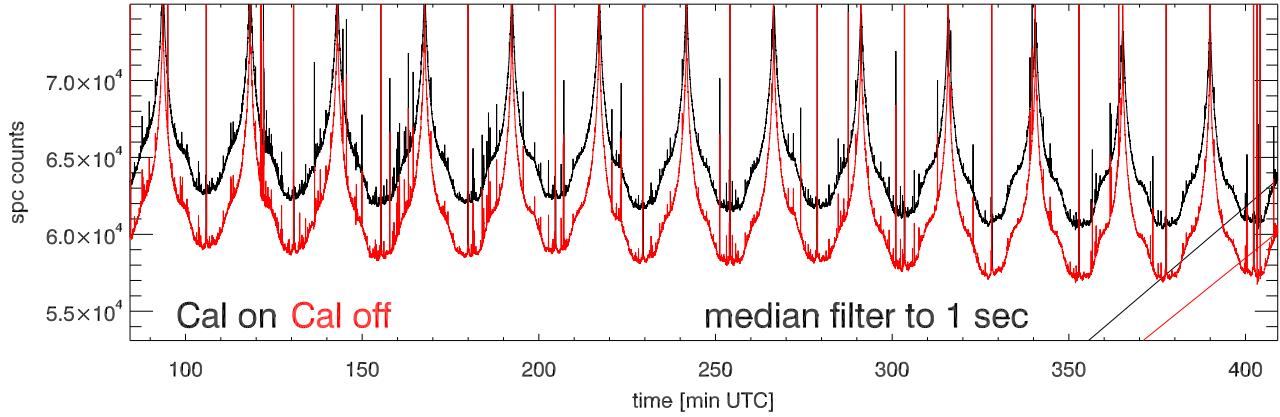
08mar13 a2030 tp vs time. Beam0A
