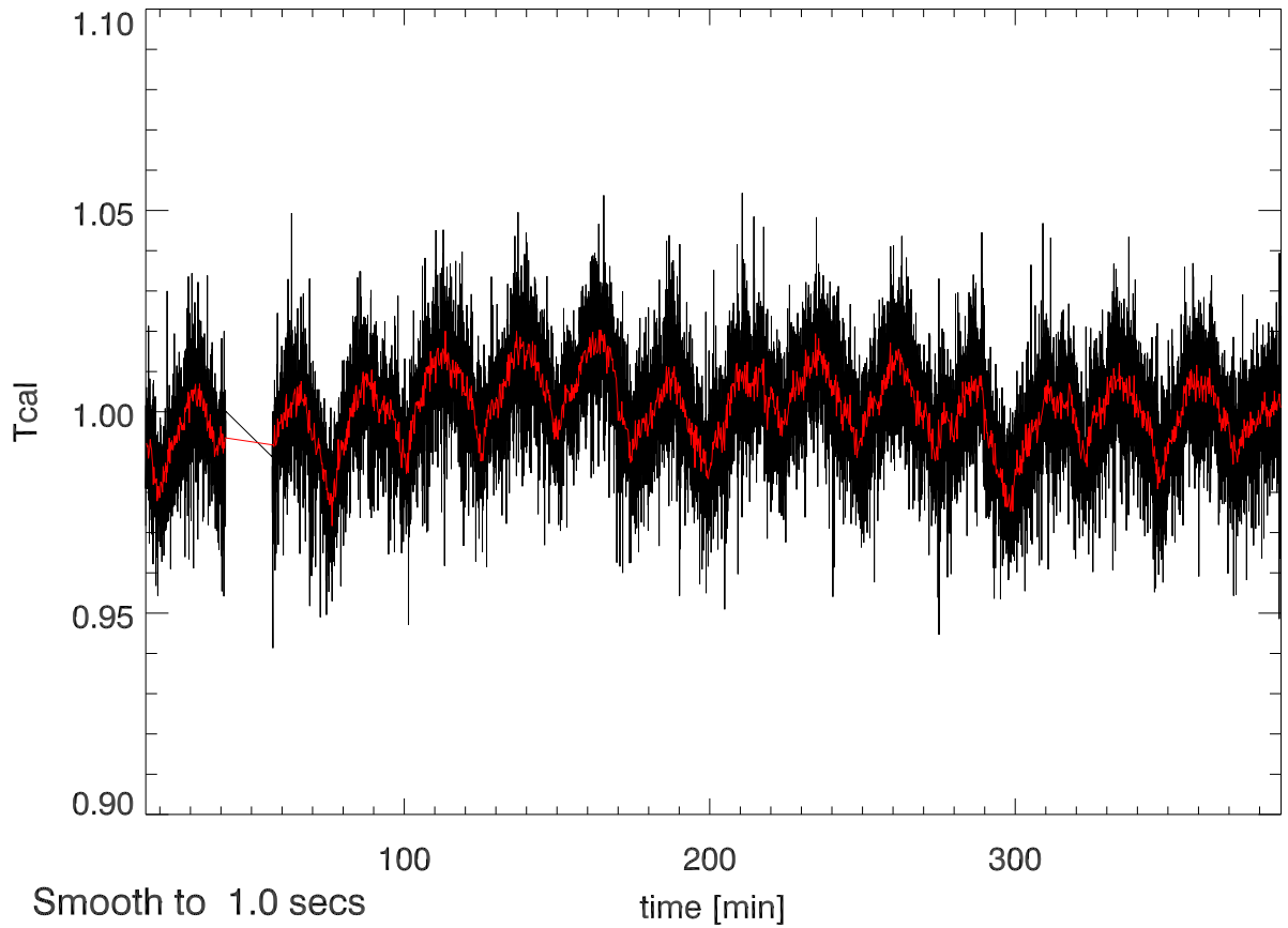
07jun12 calOn - calOff Beam0A SigA: 0.019
