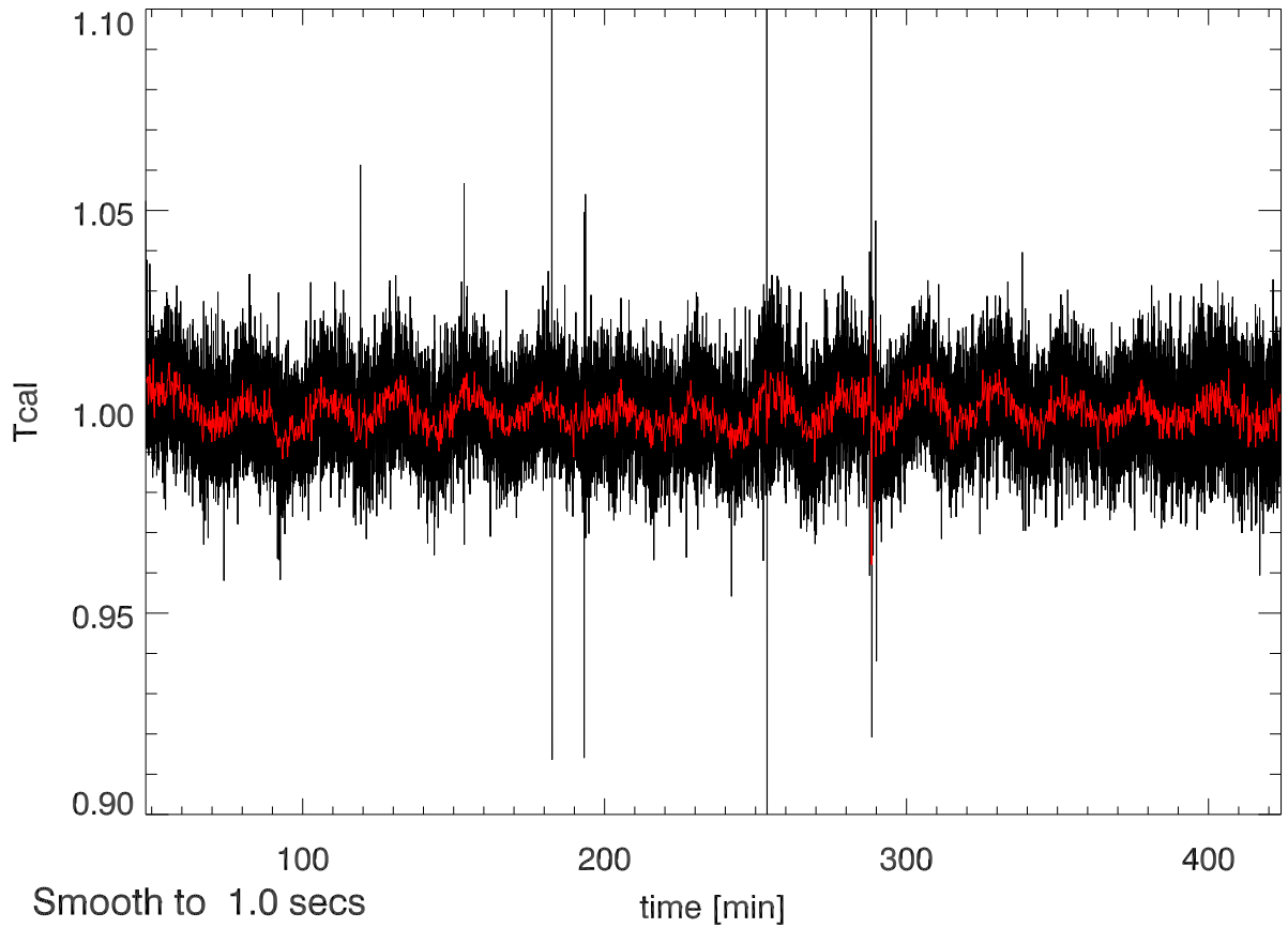
07jul11 calOn - calOff Beam0A SigA: 0.017
