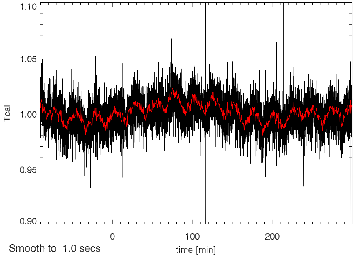
04oct12 calOn - calOff Beam0A SigA: 0.019
