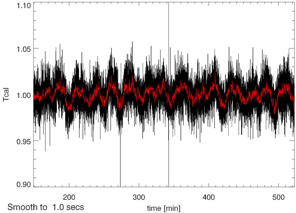
04may12 calOn - calOff Beam0A SigA: 0.023
