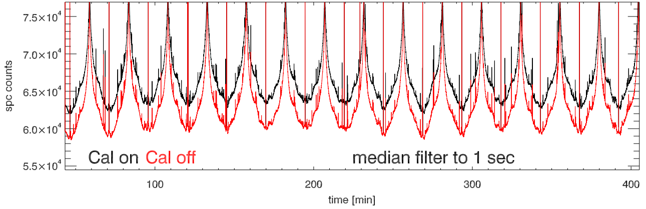
tp vs time. Beam0B
