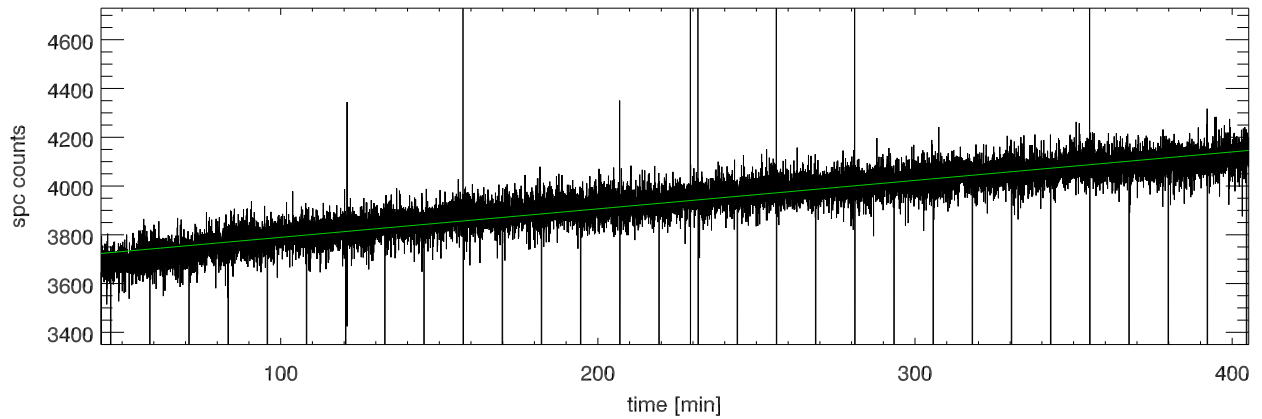
calOn - calOff Beam0B
