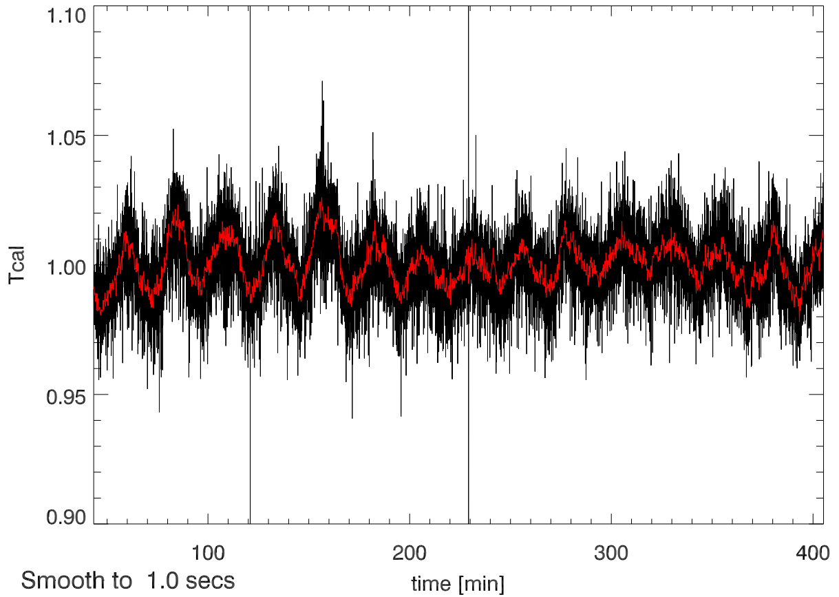
03jun12 calOn - calOff Beam0A SigA: 0.019
