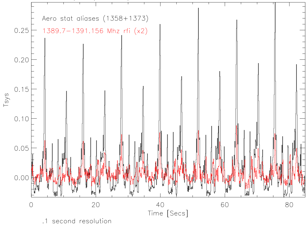
11sep09 p2473. power vs time aerostat, and 1390 rfi
