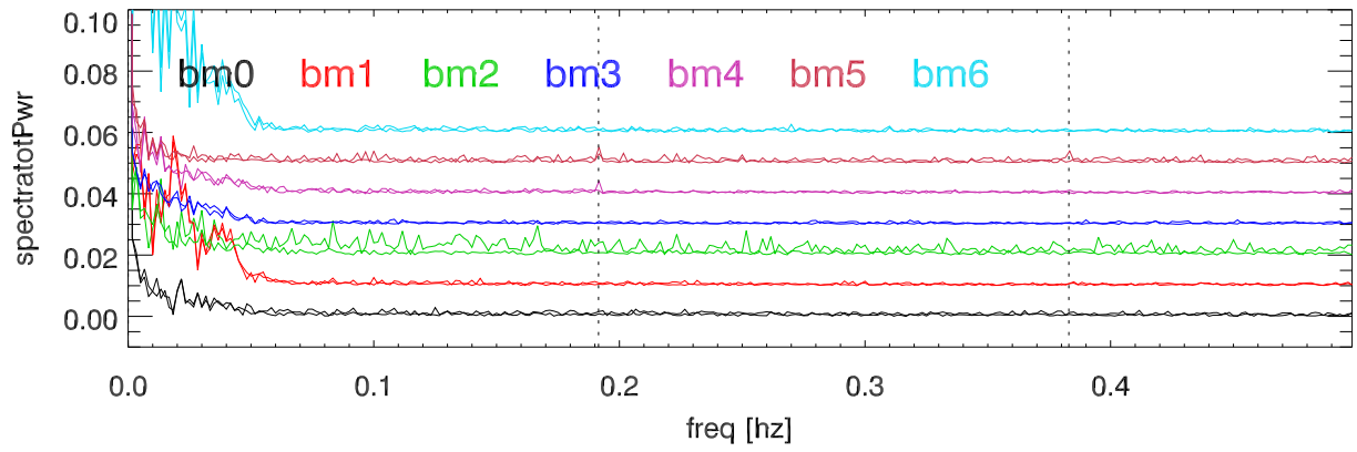
100406 Alfa spectraTotPwr. Scan:009600002
