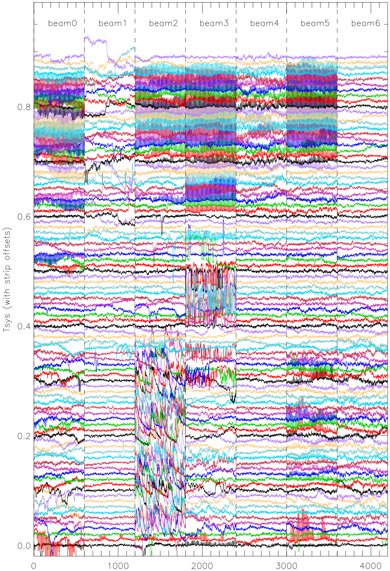
sep09 A2010 TotalPwrA/TotalPwrB by strip and beam.. bad strips
