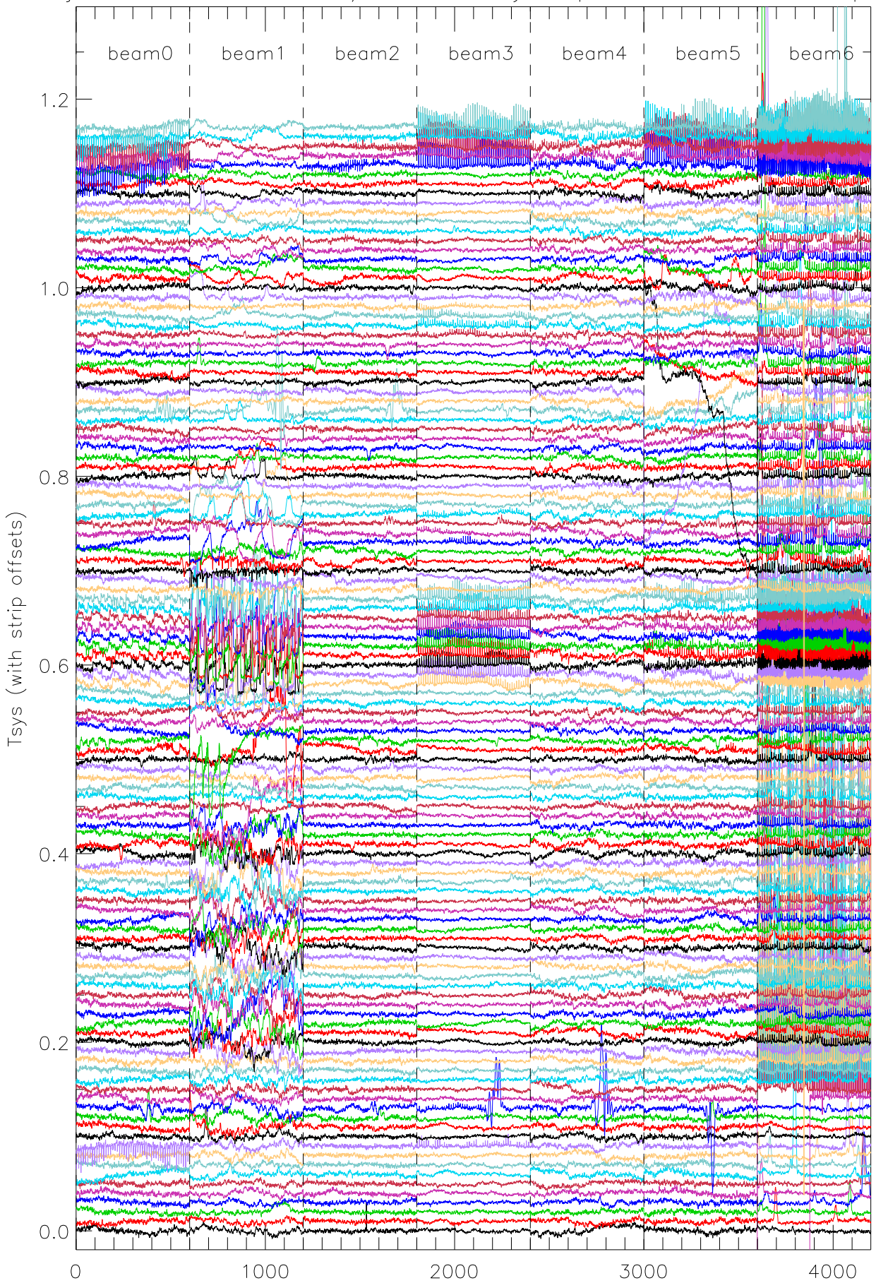
jan09 A2010 TotalPwrA/TotalPwrB by strip and beam.. bad strips
