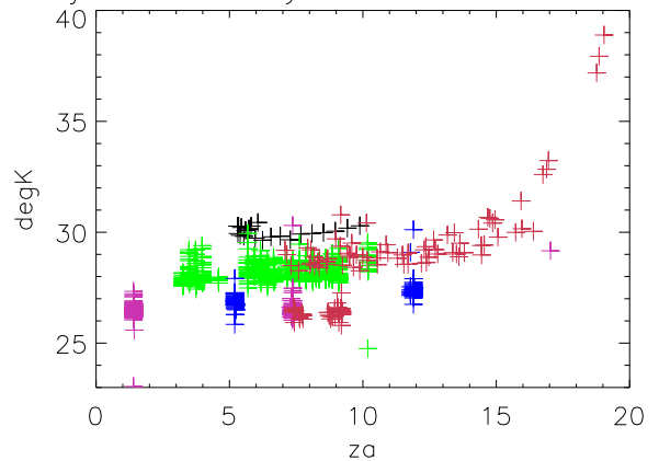
jun05 Alfa Tsys vs za Pixel 3 Pol B
