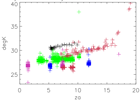
jun05 Alfa Tsys vs za Pixel 3 Pol A
