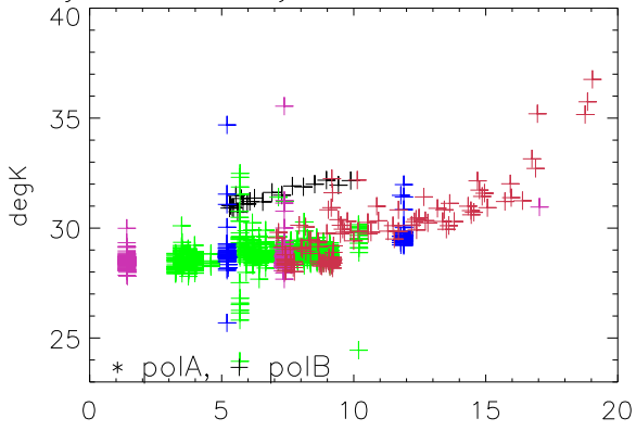
jun05 Alfa Tsys vs za Pixel 0 Pol A
