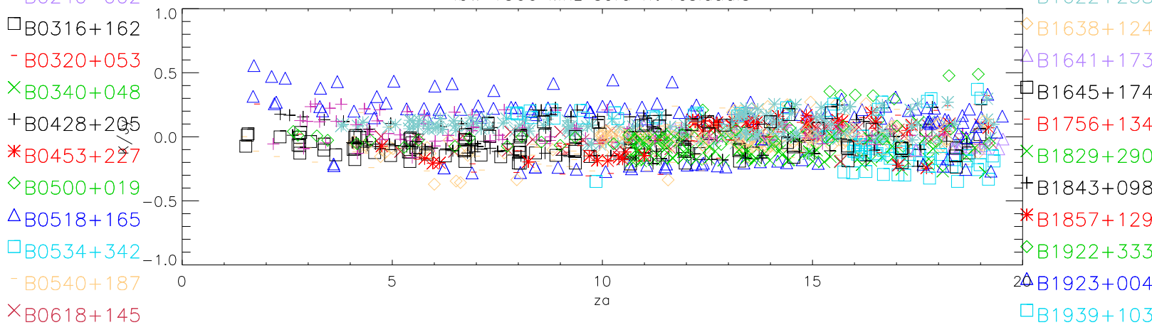
lbw 1375 Mhz sefd fit residuals
