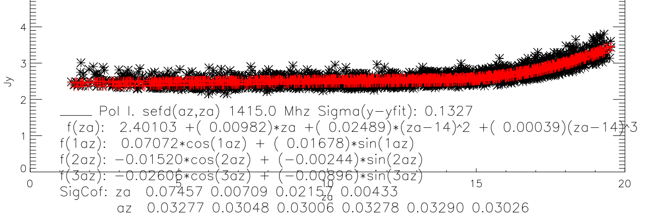
lbw 1415 sefd vs za and fit mar03-jun06
