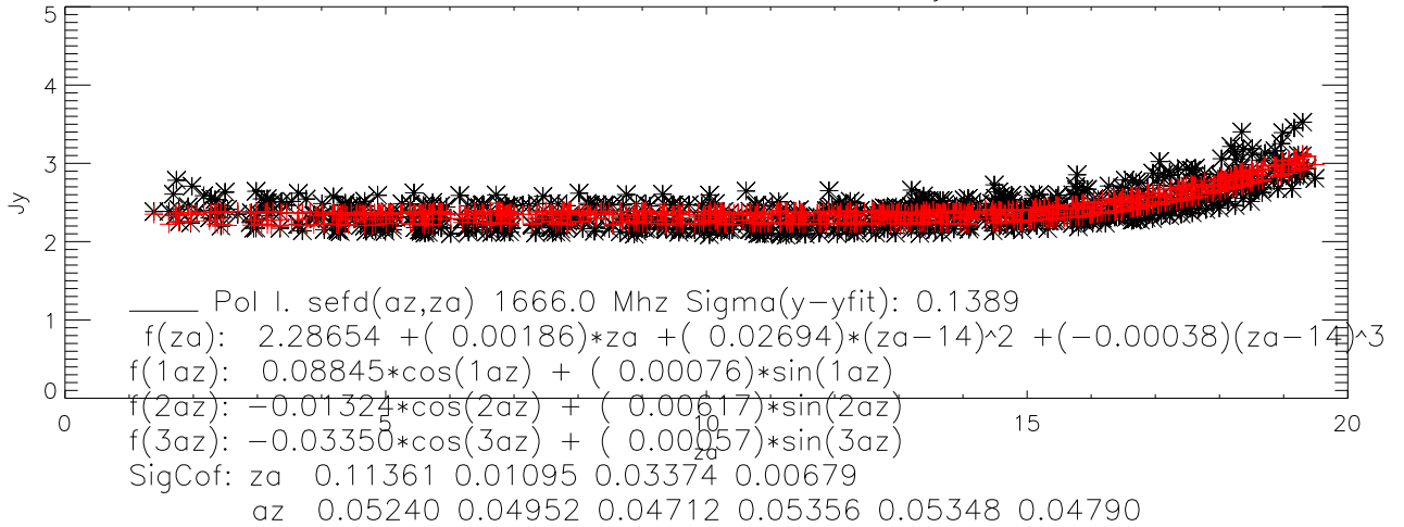
lbw 1666 sefd vs za and fit mar03-jun06
