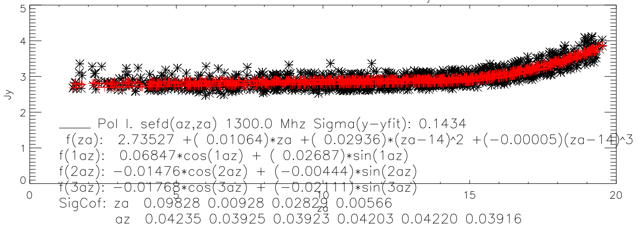
lbw 1375 sefd vs za and fit mar03-jun06
