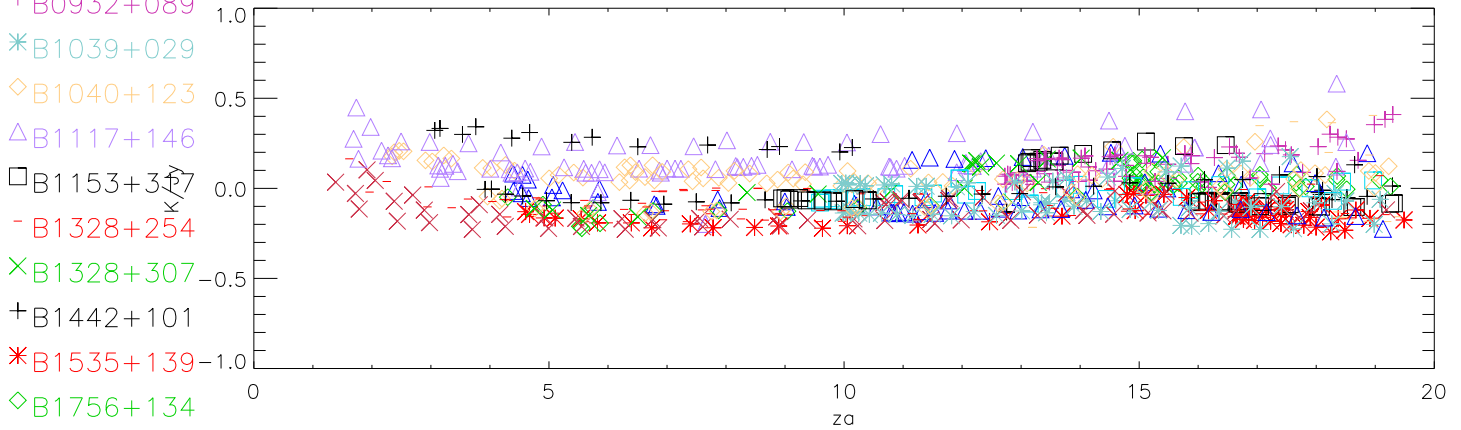
lbw 1666 Mhz sefd fit residuals
