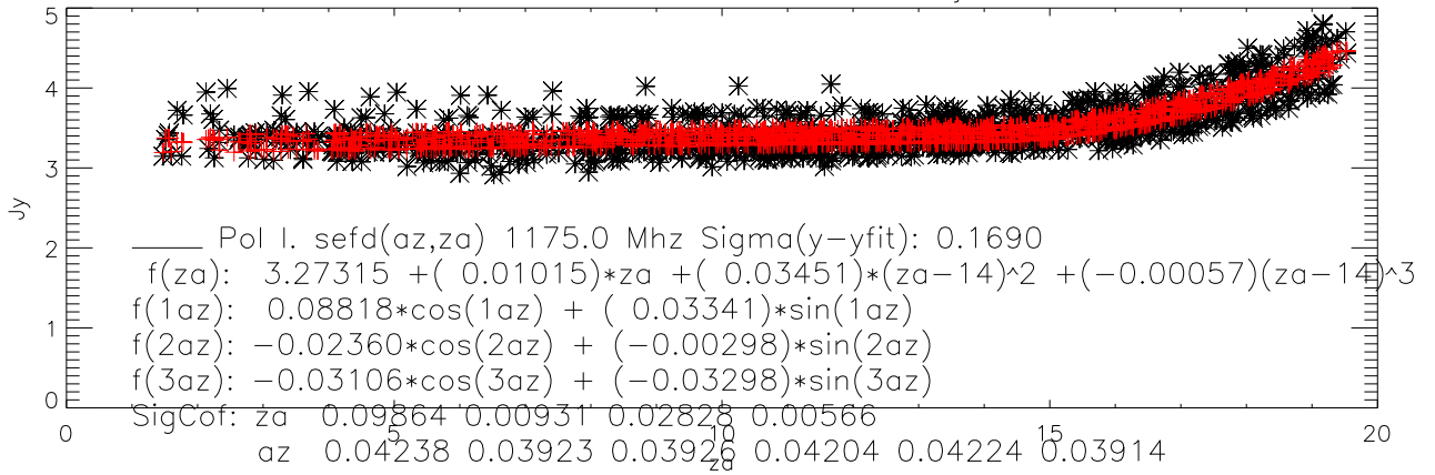
lbw 1300 sefd vs za and fit mar03-jun06
