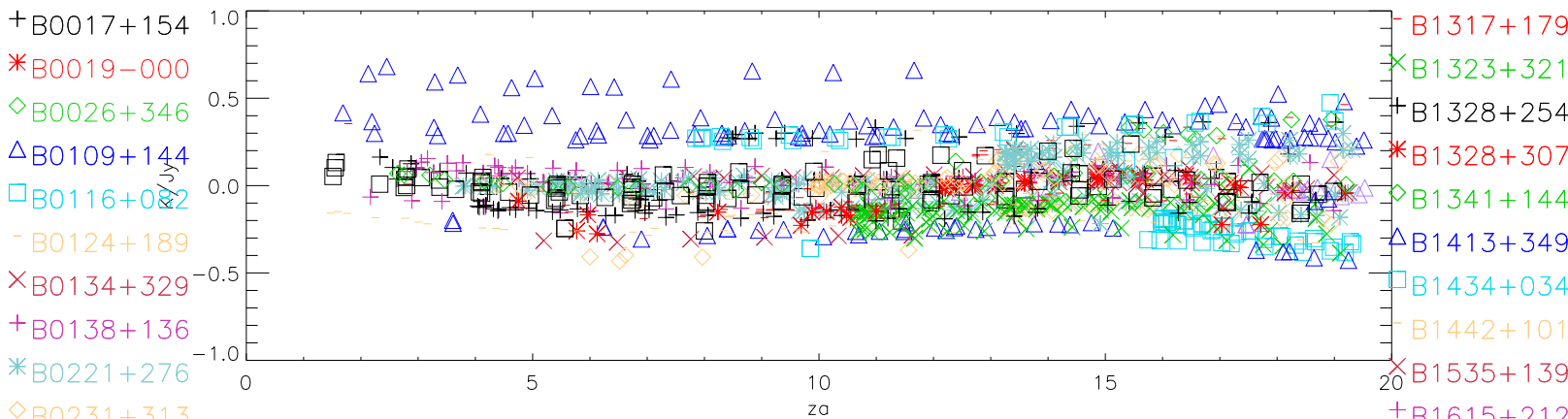
lbw 1300 Mhz sefd fit residuals
