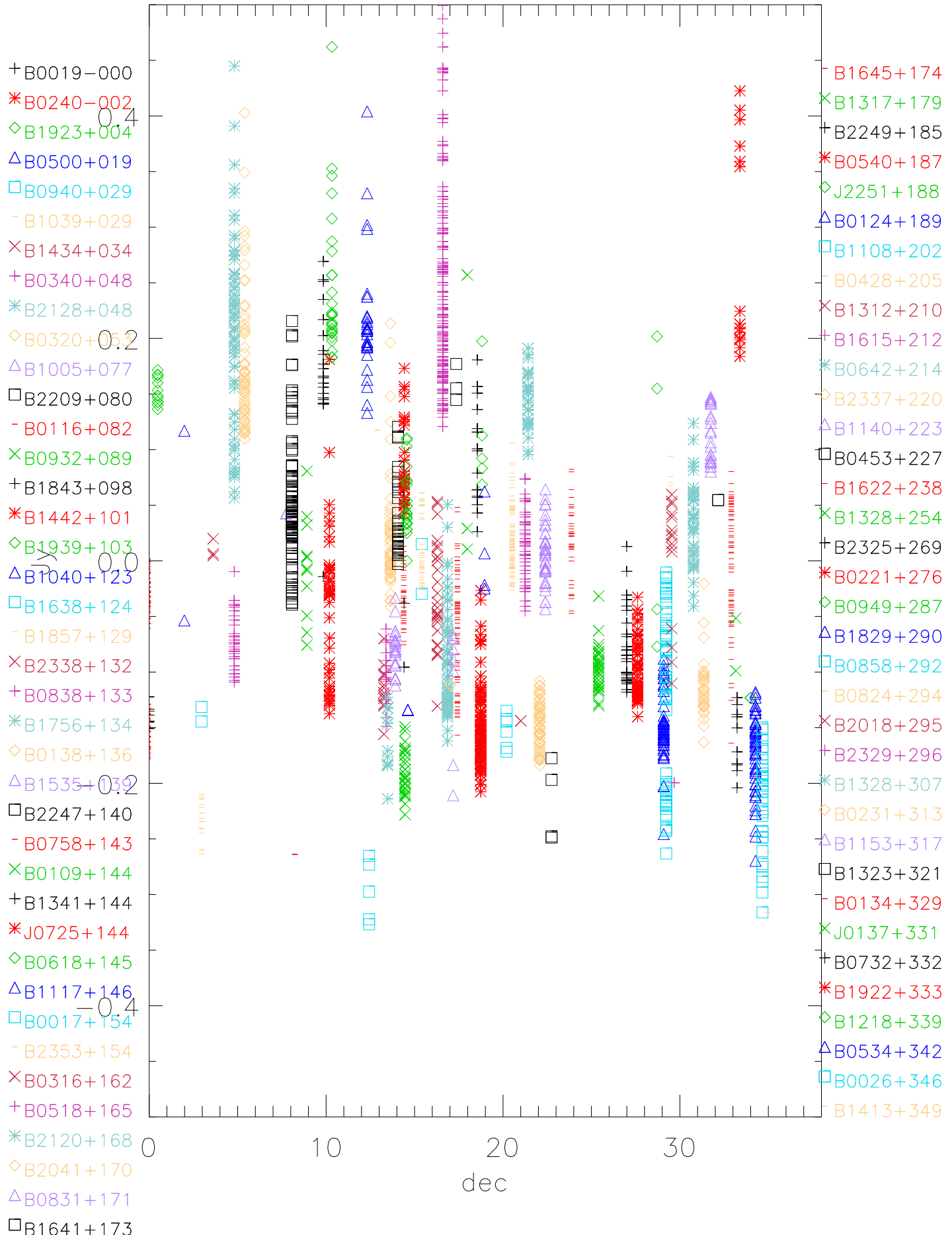
lbw 1415 Mhz sefd fit residuals by src
