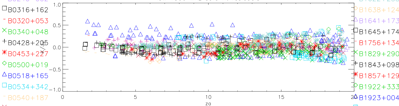
lbw 1375 Mhz sefd fit residuals
