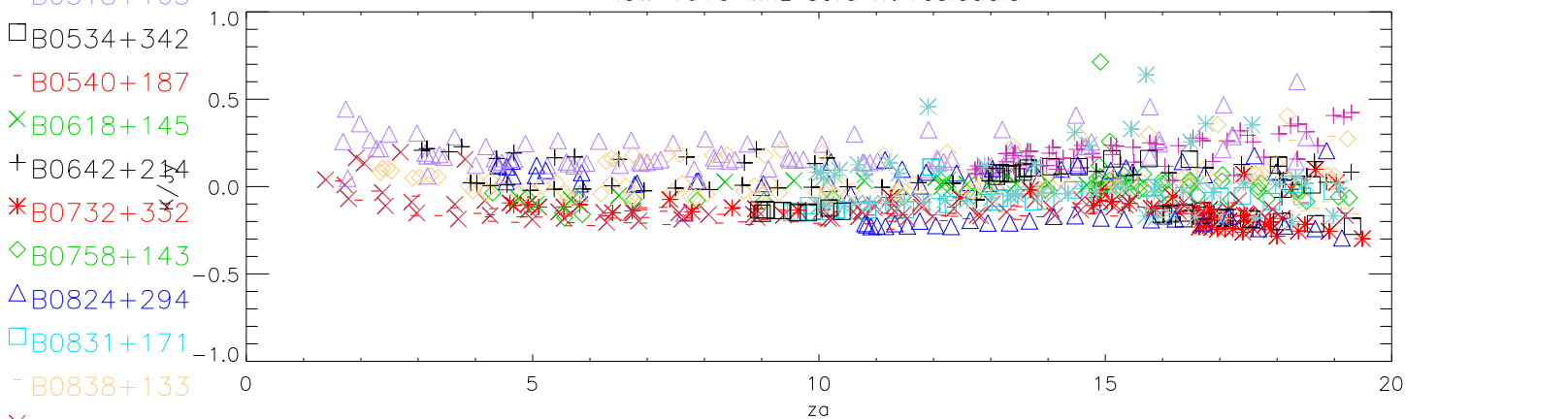
lbw 1666 Mhz sefd fit residuals
