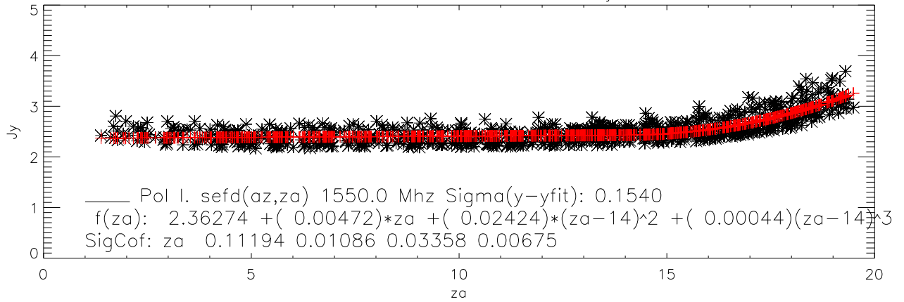
lbw 1610 sefd vs za and fit mar03-jun06
