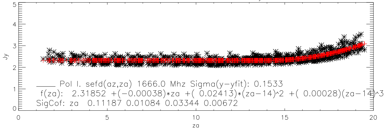
lbw 1666 sefd vs za and fit mar03-jun06
