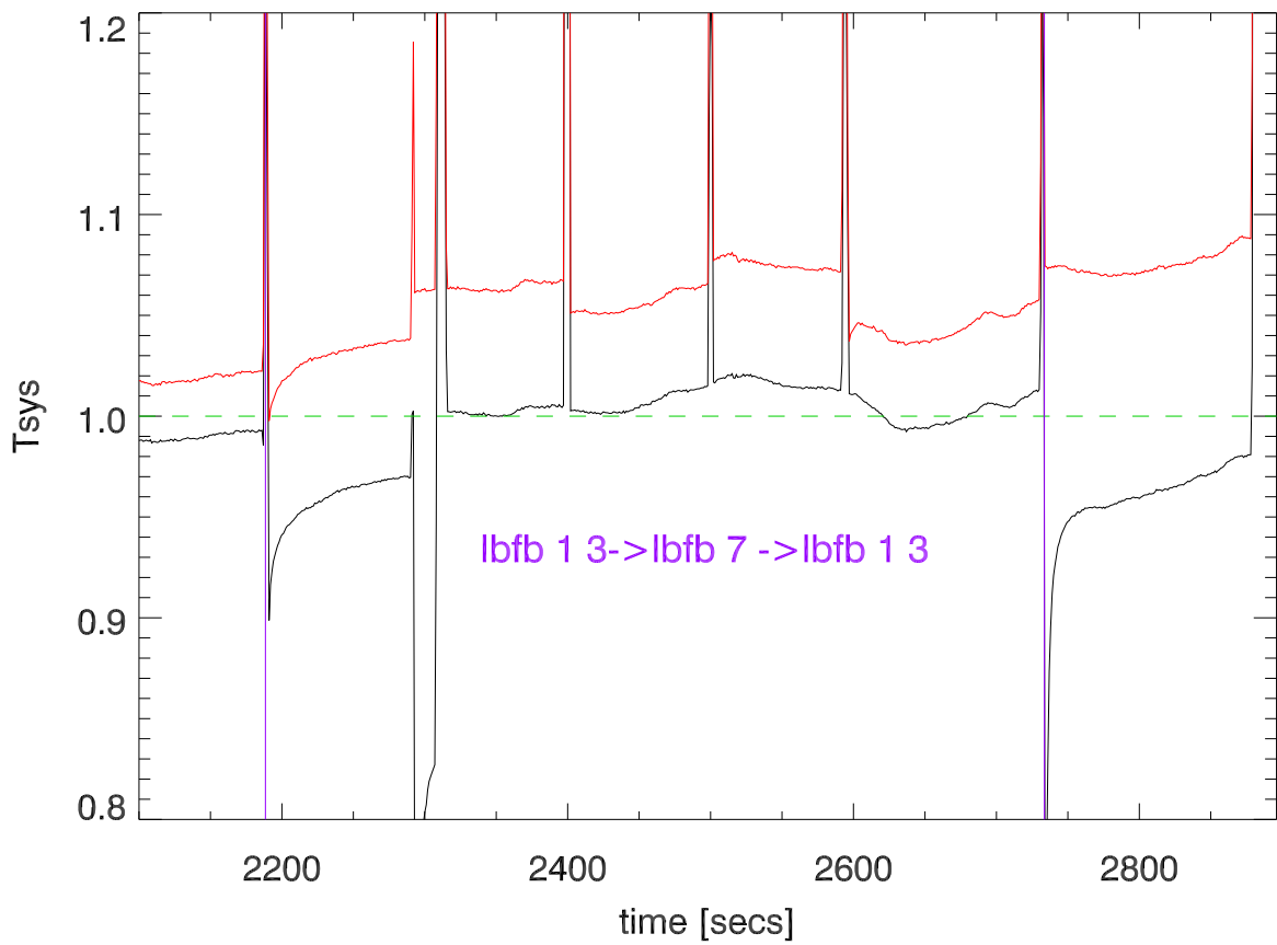
blowup around filter switches
