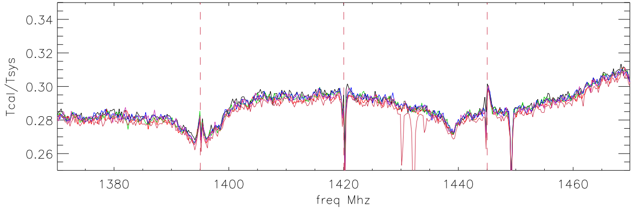
09mar06 lbw Tcal/Tsys with filter: 2 1120-1220 polA
