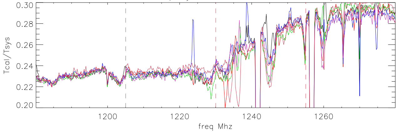
09mar06 lbw Tcal/Tsys with filter: 8 1180-1280 polB
