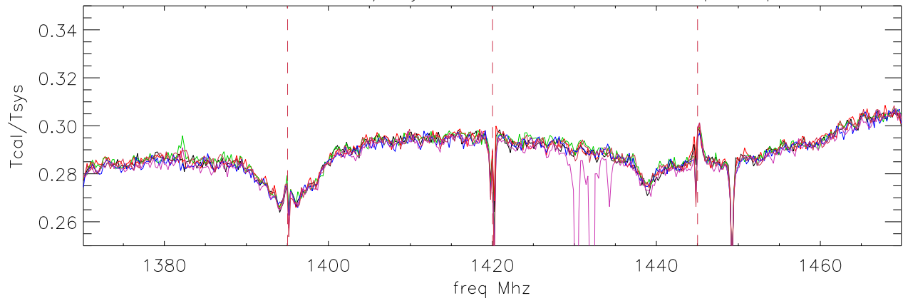
09mar06 lbw Tcal/Tsys with filter: 9,5 1280 hipass polB
