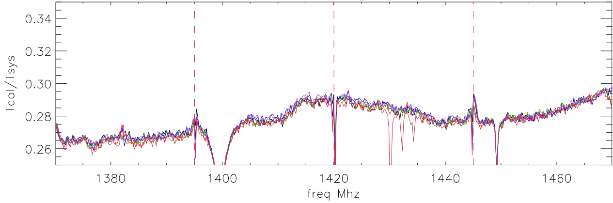
09mar06 lbw Tcal/Tsys with filter: 1,5 1370 hipass polB
