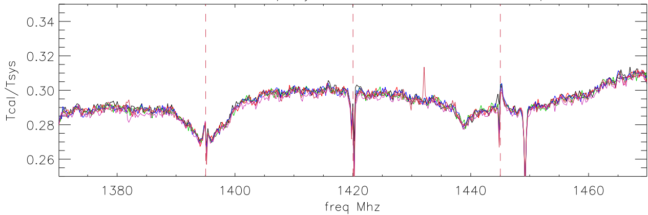
09mar06 lbw Tcal/Tsys with filter: 6 1360-1470 polA
