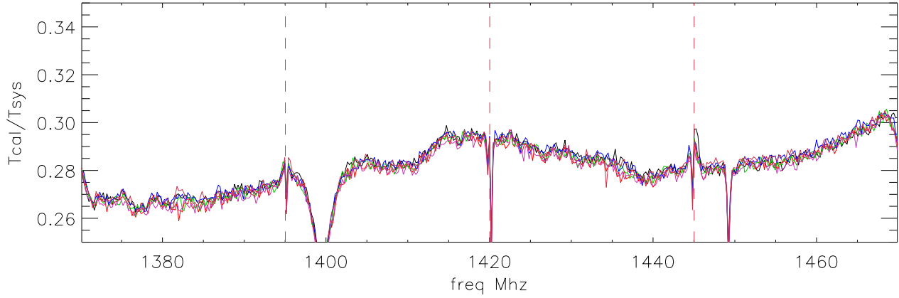
09mar06 lbw Tcal/Tsys with filter: 5 1100-1800 polB
