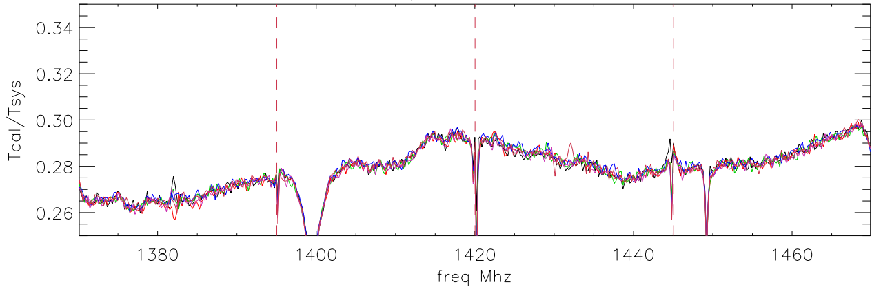
09mar06 lbw Tcal/Tsys with filter: 6 1360-1470 polB
