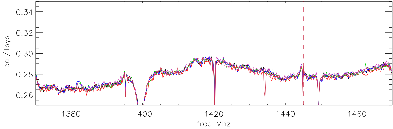
09mar06 lbw Tcal/Tsys with filter: 3 1230-1470 polB
