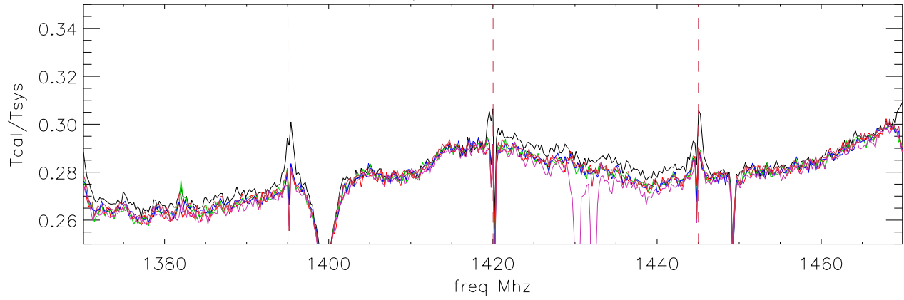
09mar06 lbw Tcal/Tsys with filter: 9,5 1280 hipass polB
