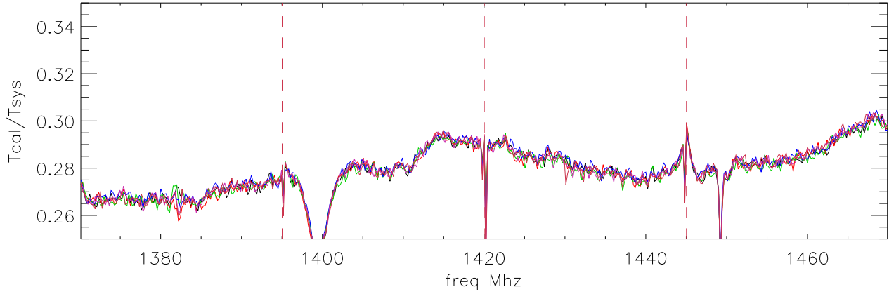
09mar06 lbw Tcal/Tsys with filter: 7 1320 hipass polB
