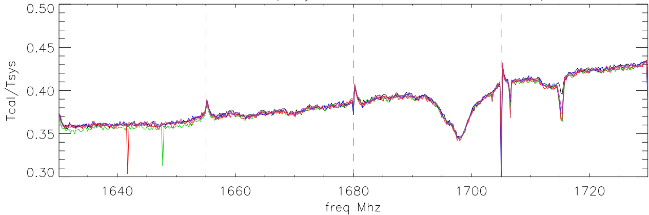
09mar06 lbw Tcal/Tsys with filter: 4 1550-1820 polB
