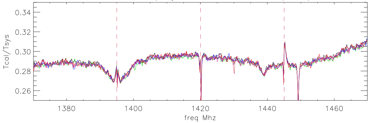
09mar06 lbw Tcal/Tsys with filter: 8 1180-1280 polA
