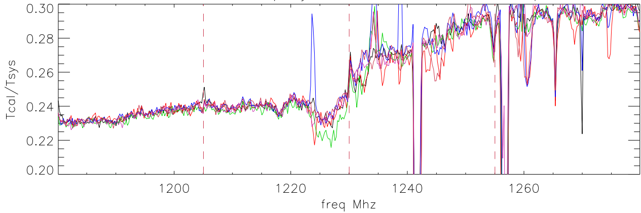
09mar06 lbw Tcal/Tsys with filter: 8 1180-1280 polB
