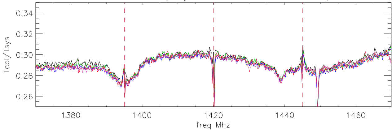
09mar06 lbw Tcal/Tsys with filter: 4 1550-1820 polA
