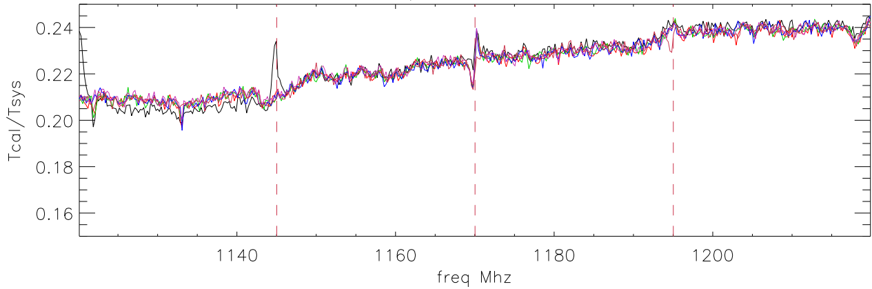
09mar06 lbw Tcal/Tsys with filter: 2 1120-1220 polB
