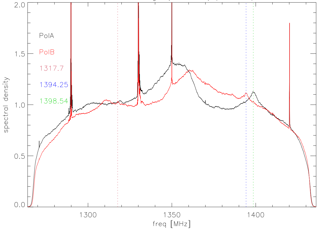
16mar10 lbw average (250secs) power spectra
