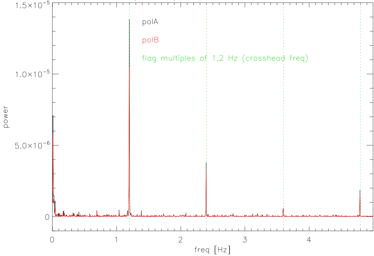
16mar10 lbw power spectrum of 4 Mhz about 1317.7 MHz
