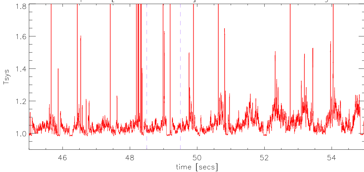
total power [1211–1225 MHz] vs time. .001 second averages
