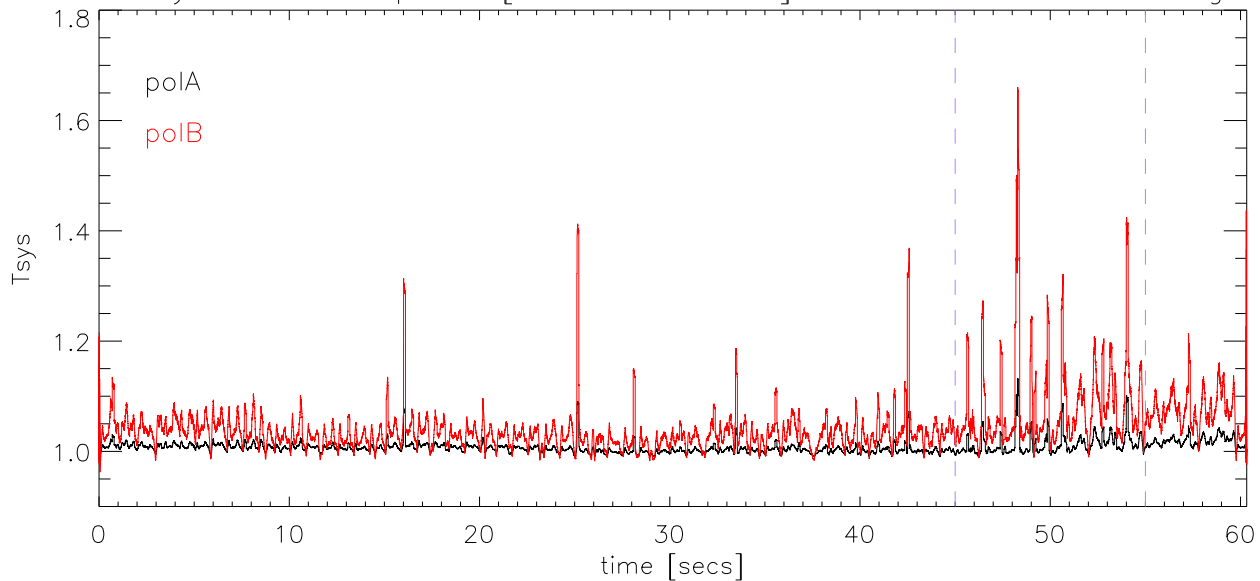
total power [1211–1225 MHz] vs time. .01 second averages
