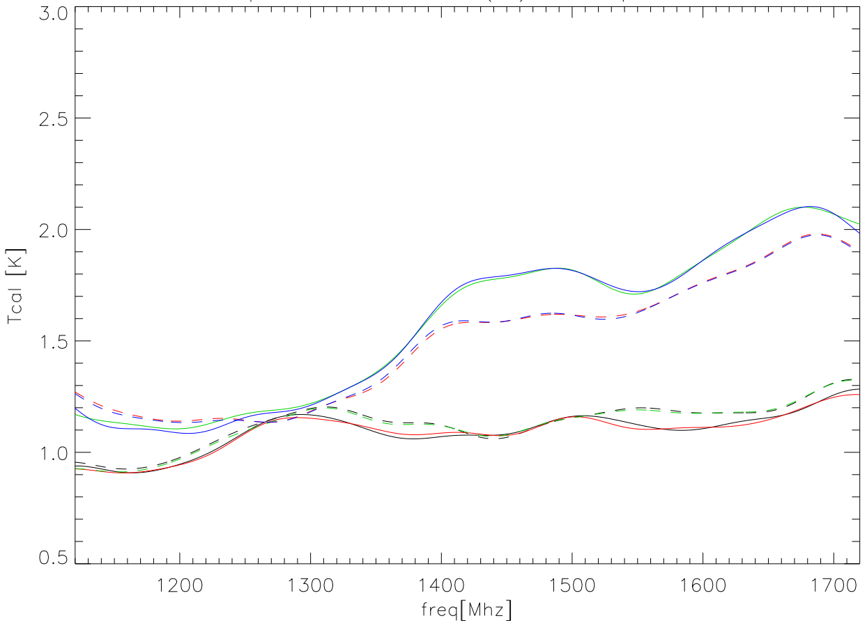
26sep08 Cal In Kelvins (fit) vs freq Low cal
