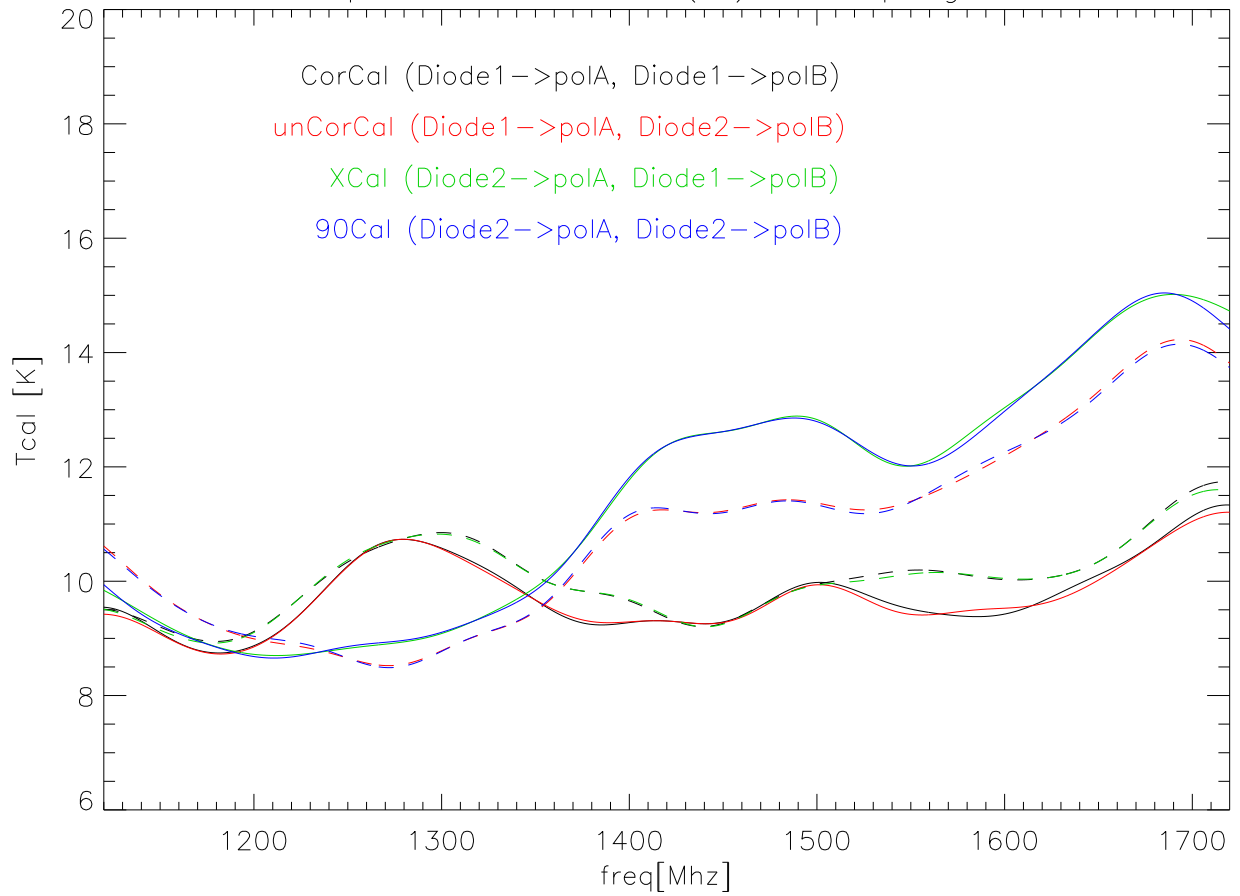
26sep08 Cal In Kelvins (fit) vs freq Low cal
