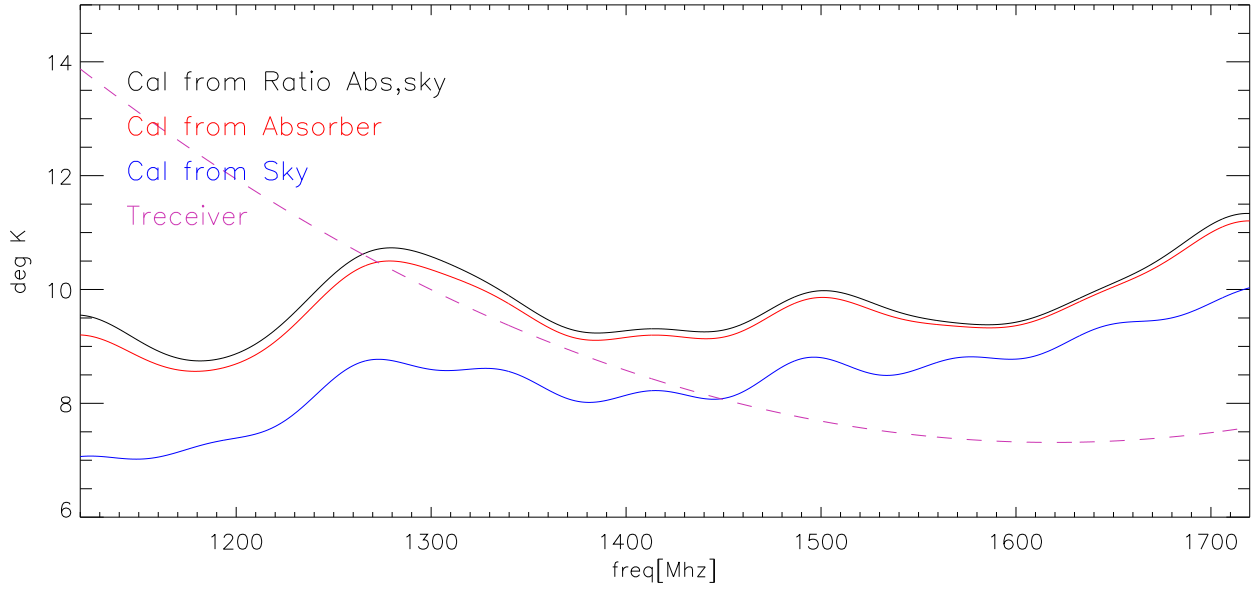
26sep08 Cal in Kelvins vs freq polB
