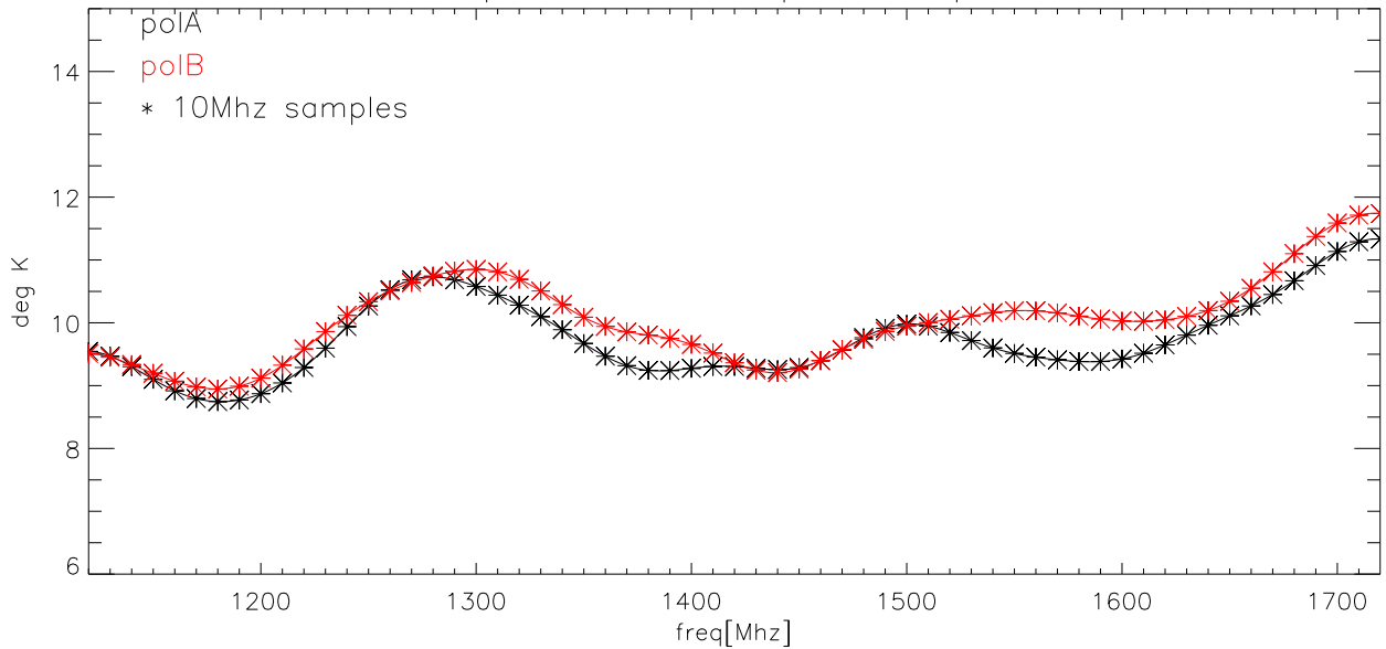
26sep08 Cal in Kelvins polA,B overplotted
