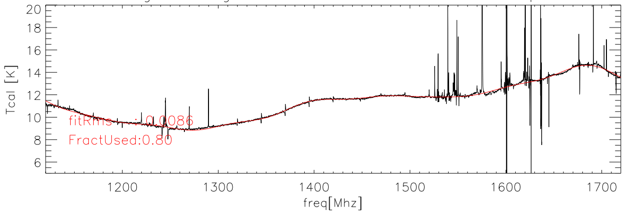
29aug08 Averaged data and fit for Tcal Kelvins hxcal polA
