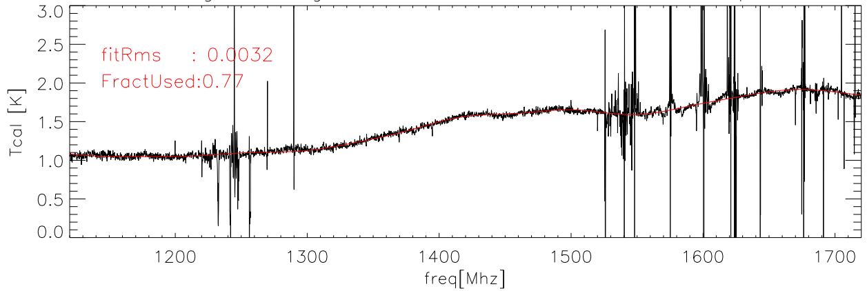
29aug08 Averaged data and fit for Tcal Kelvins lxcal polB
