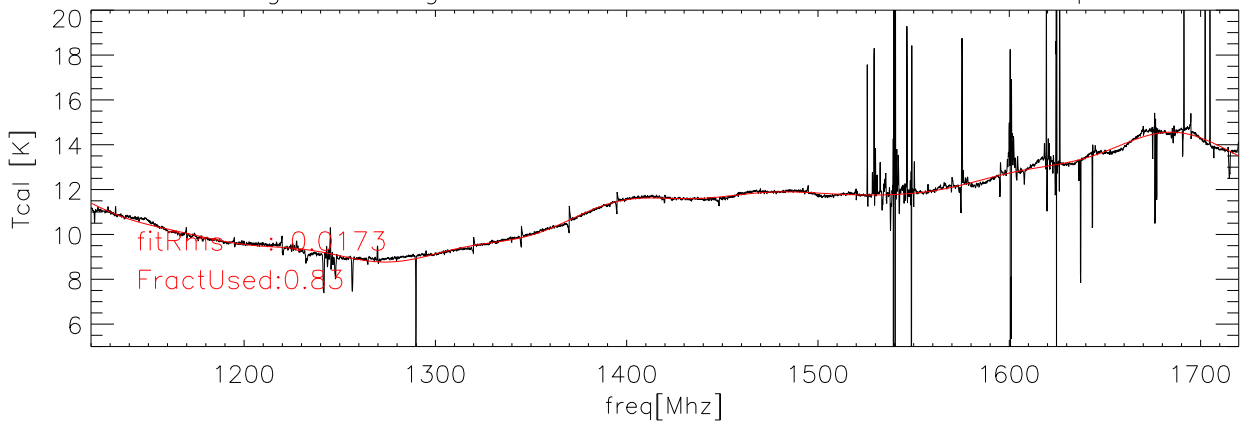
29aug08 Averaged data and fit for Tcal Kelvins lcor polA
