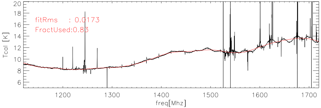
29aug08 Averaged data and fit for Tcal Kelvins h90cal polB
