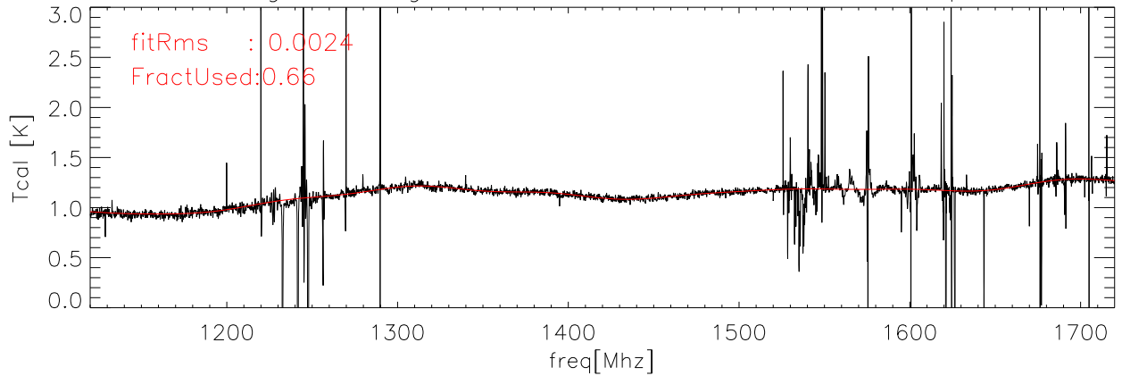
29aug08 Averaged data and fit for Tcal Kelvins lcor polB
