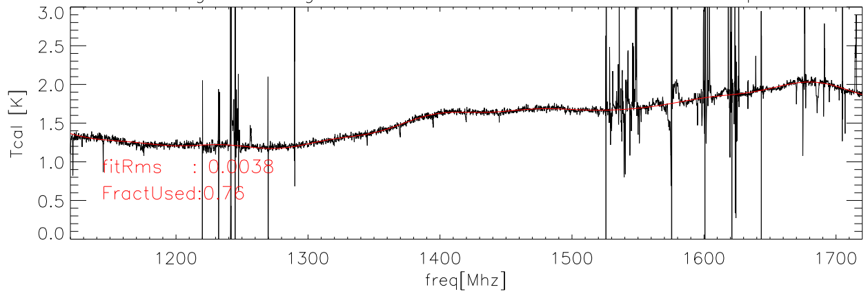
29aug08 Averaged data and fit for Tcal Kelvins I90cal polB
