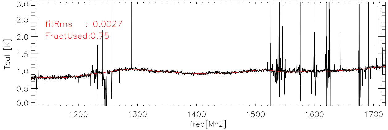
29aug08 Averaged data and fit for Tcal Kelvins lcal polB
