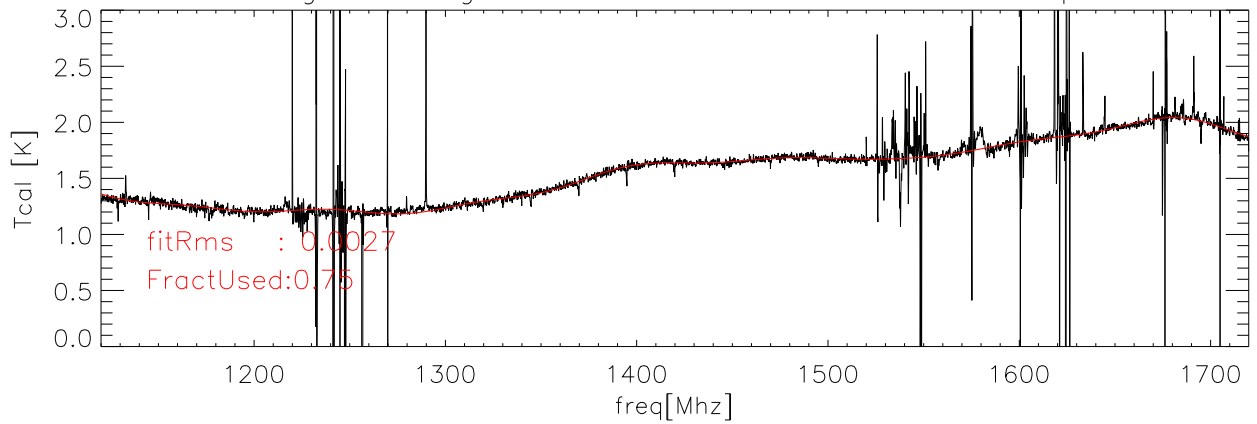
29aug08 Averaged data and fit for Tcal Kelvins lxcal polA
