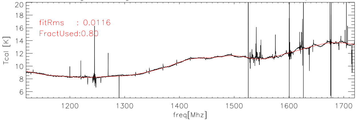
29aug08 Averaged data and fit for Tcal Kelvins hxcal polB
