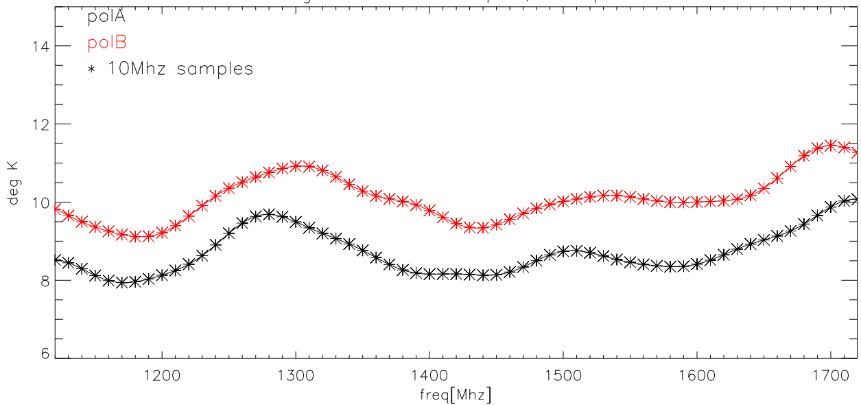
29aug08 Cal in Kelvins polA,B overplotted
