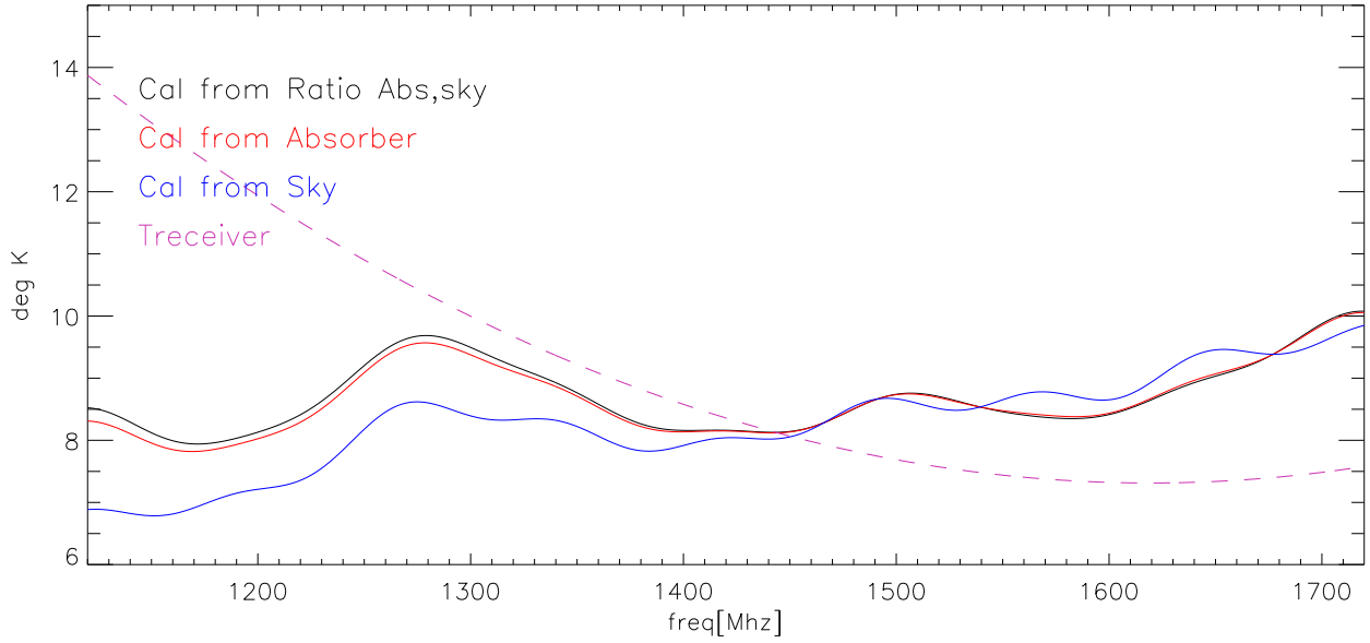
29aug08 Cal in Kelvins vs freq polB
