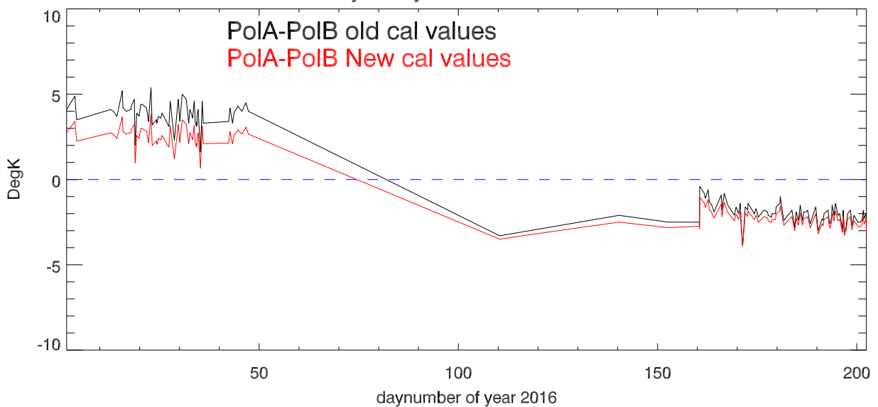
LBW 2016 TsysA-TsysB with old and new calValues
