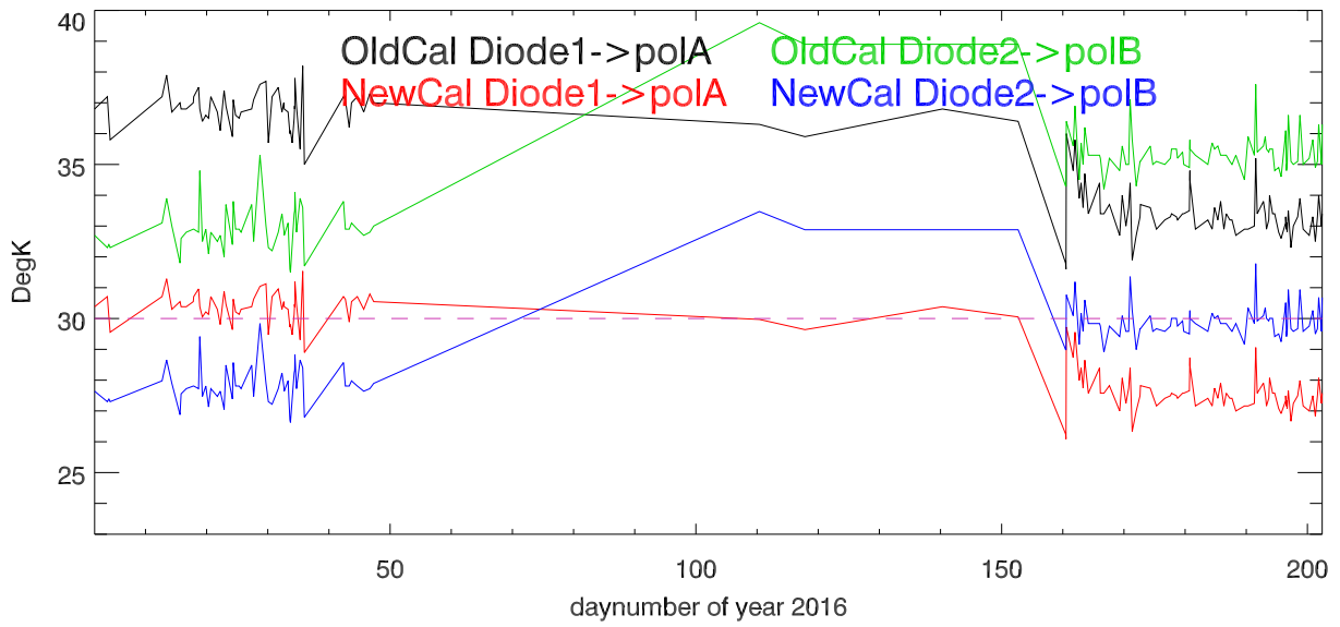
Tsys LBW 2016 Compare old,new cal values. Hcal
