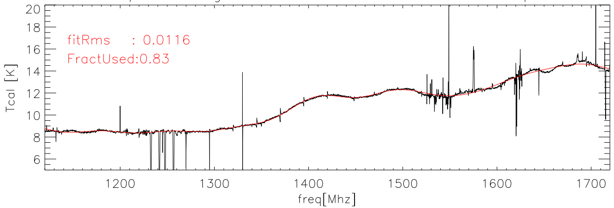
22apr07 Averaged data and fit for Tcal Kelvins hxcal polB
