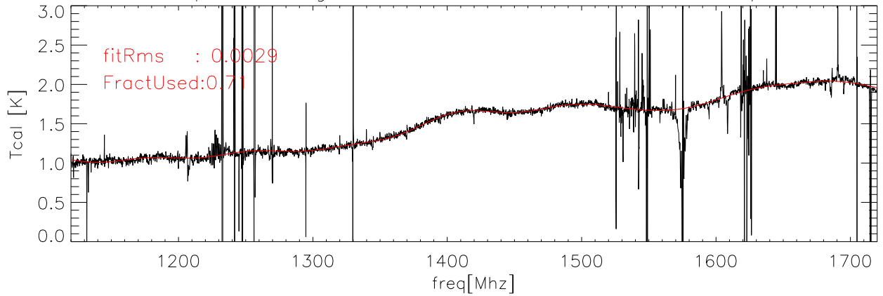
22apr07 Averaged data and fit for Tcal Kelvins lxcal polB
