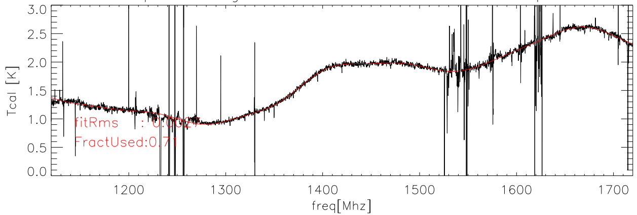
22apr07 Averaged data and fit for Tcal Kelvins lxcal polA
