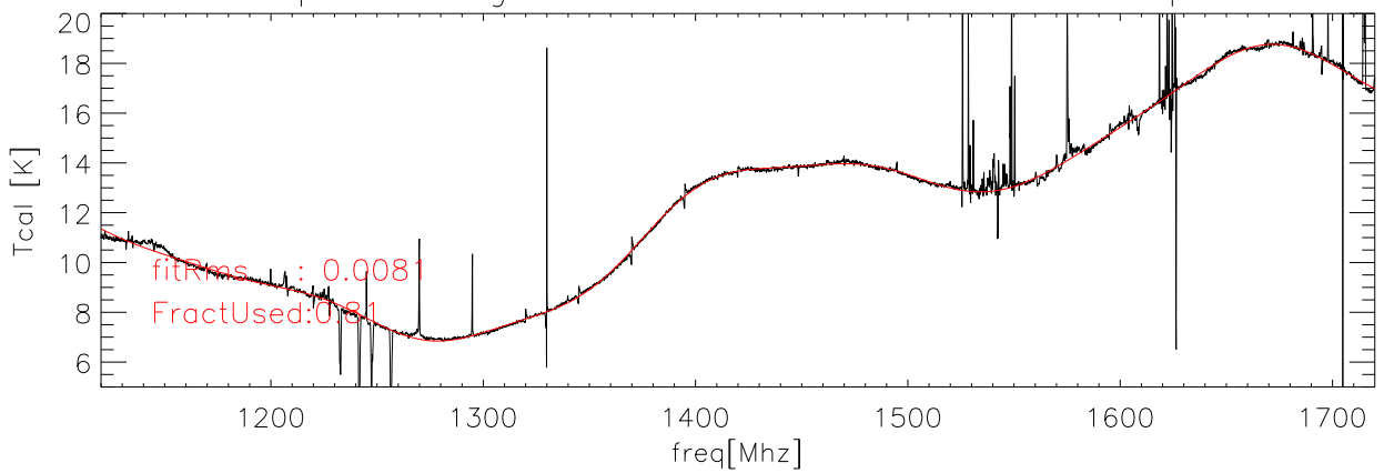
22apr07 Averaged data and fit for Tcal Kelvins hxcal polA
