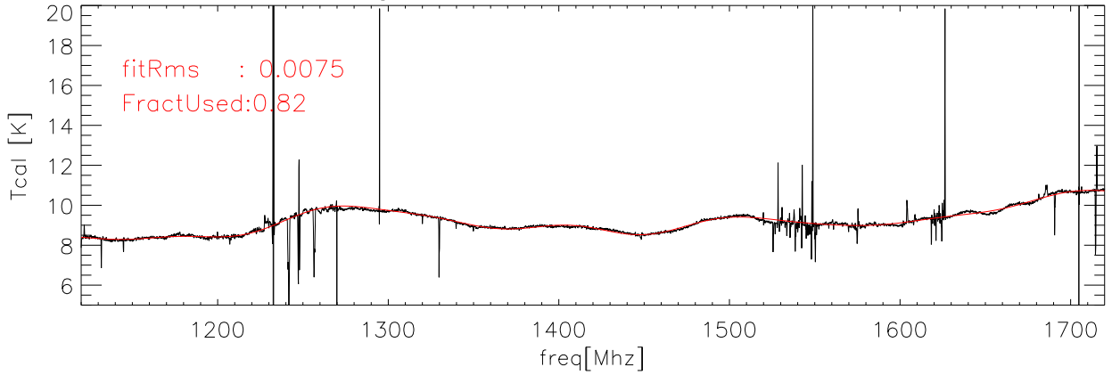
22apr07 Averaged data and fit for Tcal Kelvins h90cal poIB
