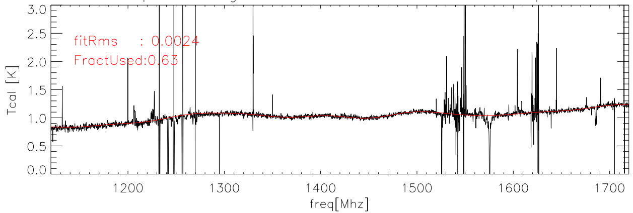
22apr07 Averaged data and fit for Tcal Kelvins lcor poIB
