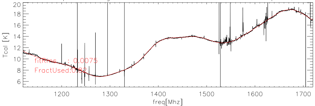
22apr07 Averaged data and fit for Tcal Kelvins lcor poIA
