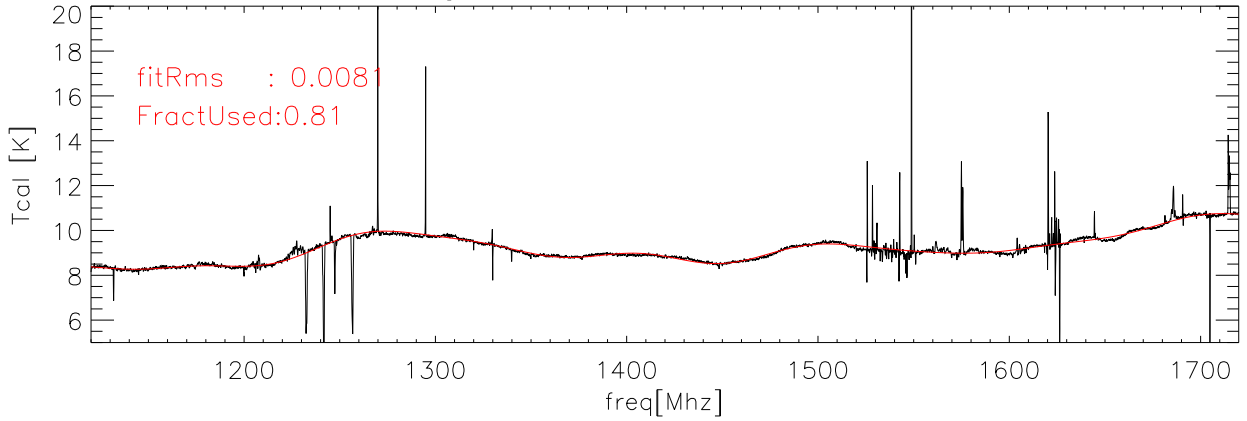
22apr07 Averaged data and fit for Tcal Kelvins hcal polB
