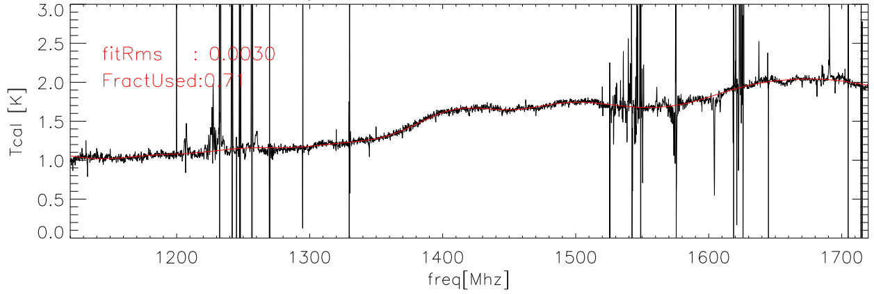
22apr07 Averaged data and fit for Tcal Kelvins I90cal polB
