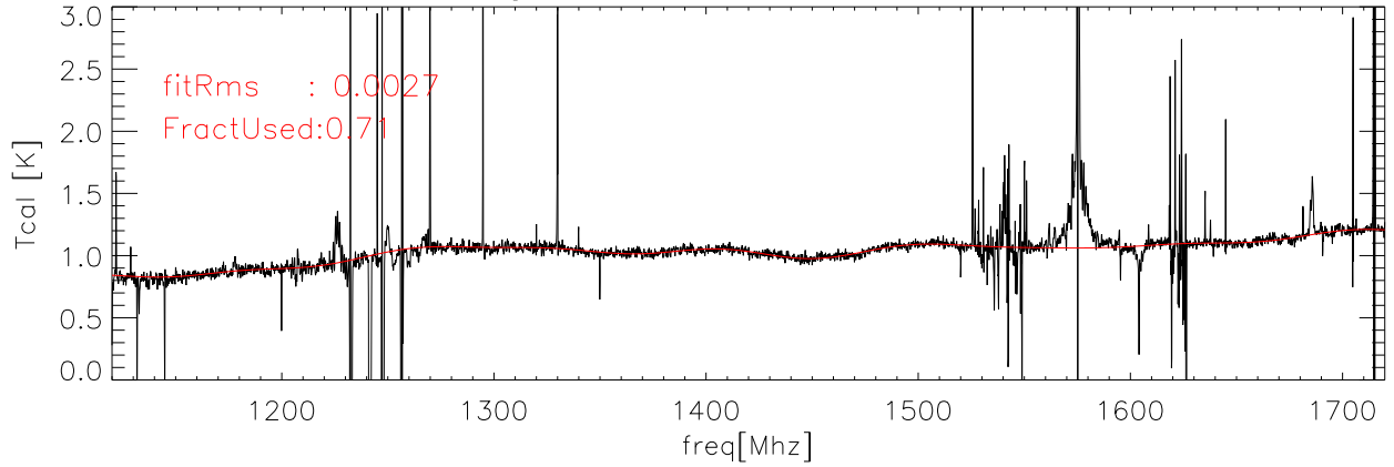
22apr07 Averaged data and fit for Tcal Kelvins lcal polB
