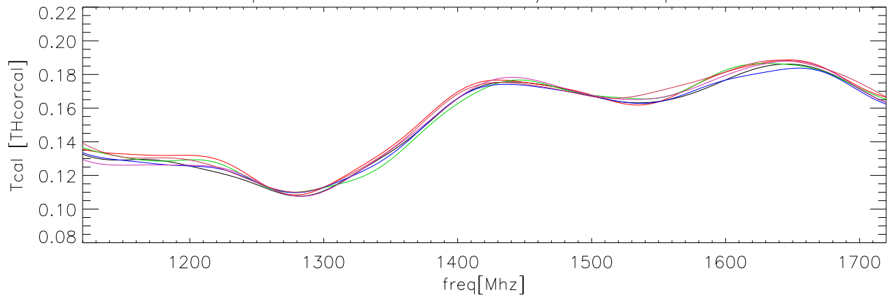
22apr07 OverPlot fits to TCal/Thcorcal polA lxccl
