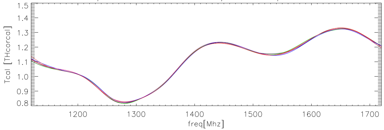
22apr07 OverPlot fits to TCal/Thcorcal poIA lcor
