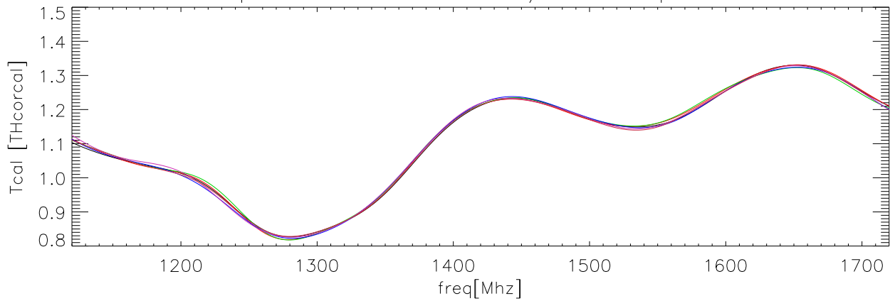
22apr07 OverPlot fits to TCal/Thcorcal polA hxccl
