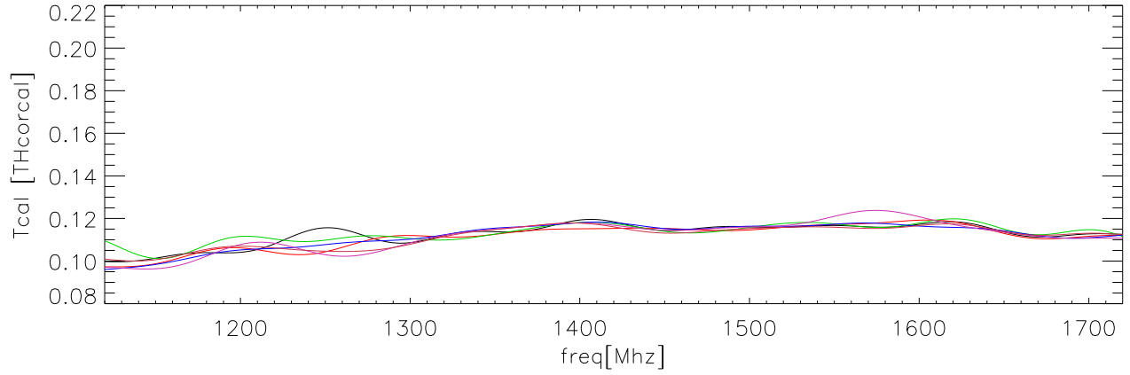
22apr07 OverPlot fits to TCal/Thcorcal polB lcal
