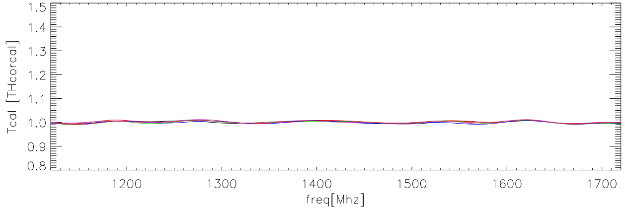
22apr07 OverPlot fits to TCal/Thcorcal poIB h90cal
