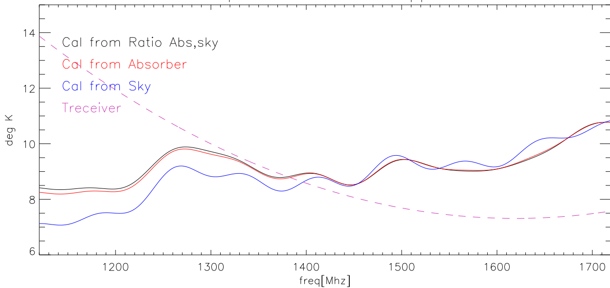
22apr07 Cal in Kelvins vs freq polB
