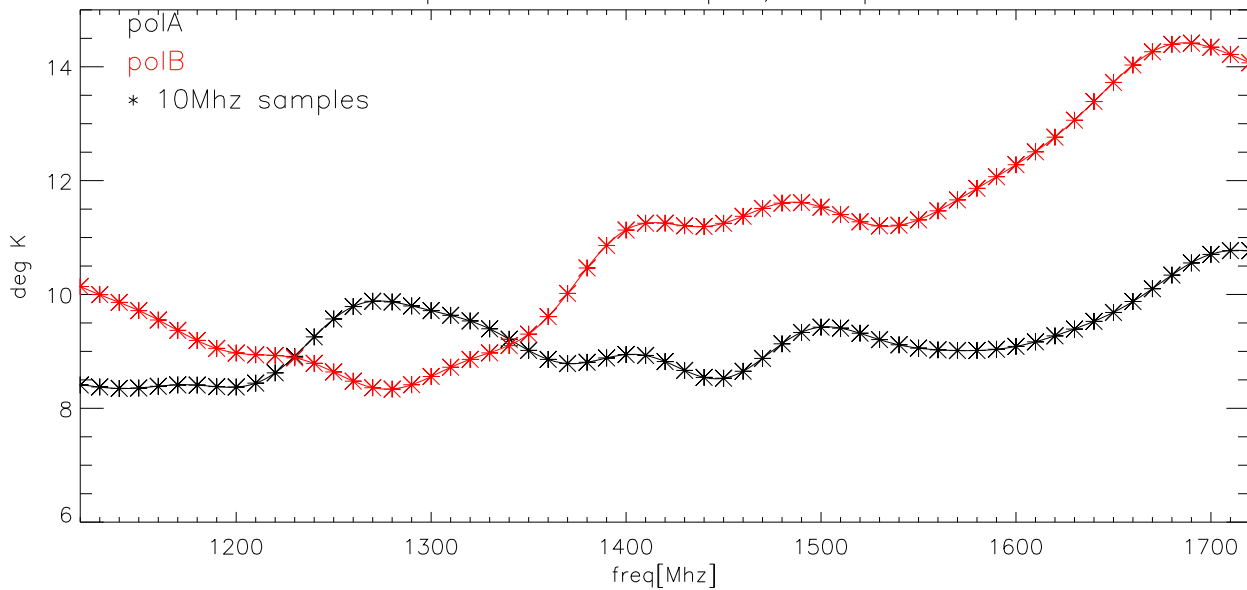
22apr07 Cal in Kelvins polA,B overplotted
