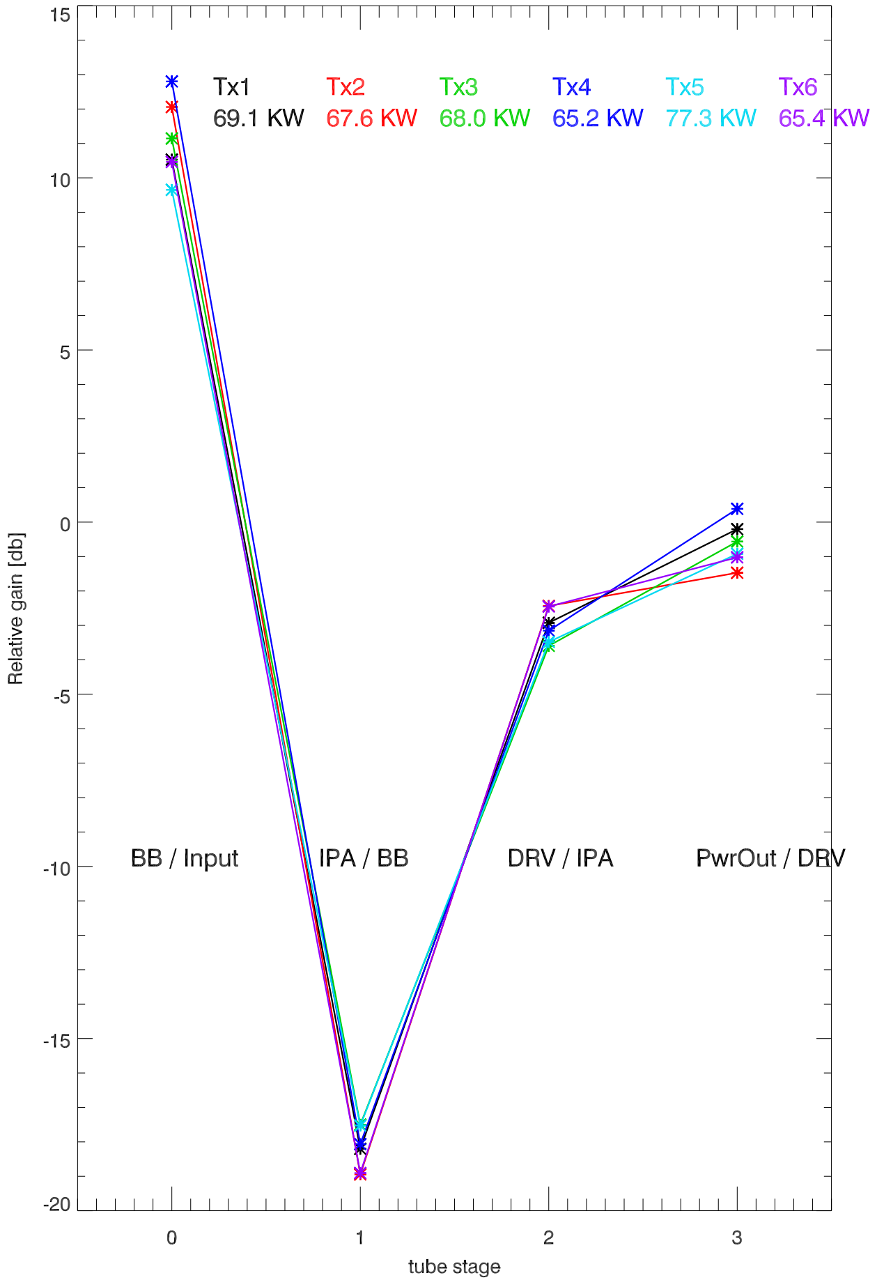
170223 relative gain of tube stages. (PwrOut[n+1]/PwrOut[n])
