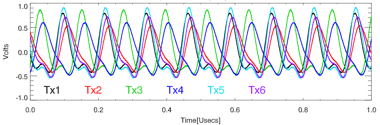
170223 overplot tube output ports. IPA Anode
