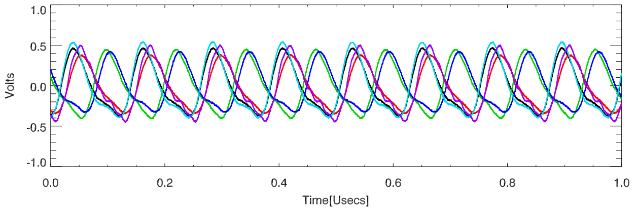
170223 overplot tube output ports. Driver Anode
