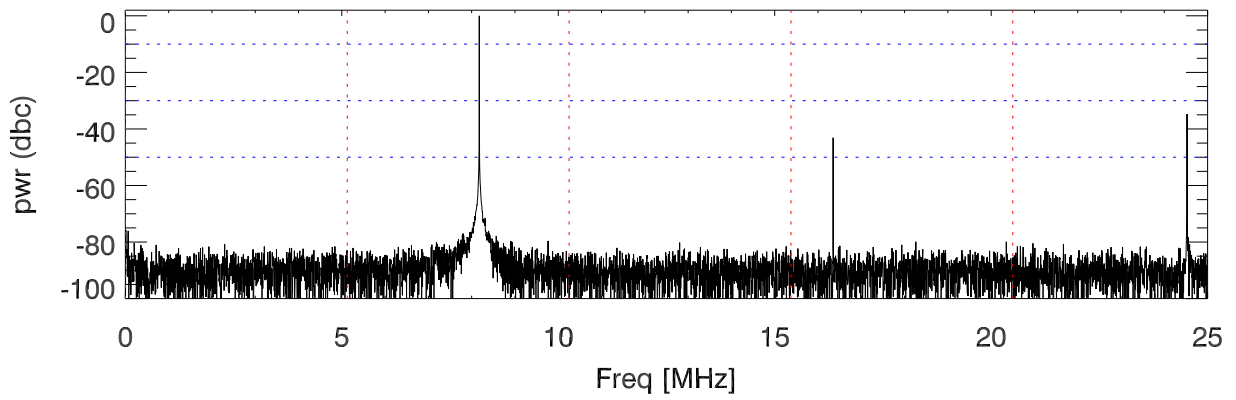
170223 tx1 tube monitor ports: spectral density. BroadBand
