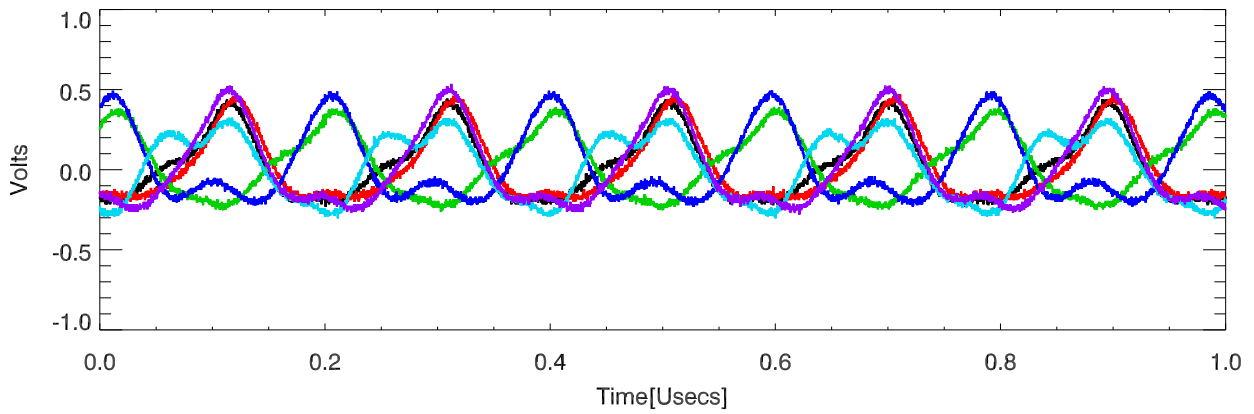
151102 overplot tube output ports. Driver Anode
