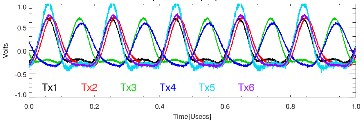
151102 overplot tube output ports. IPA Anode
