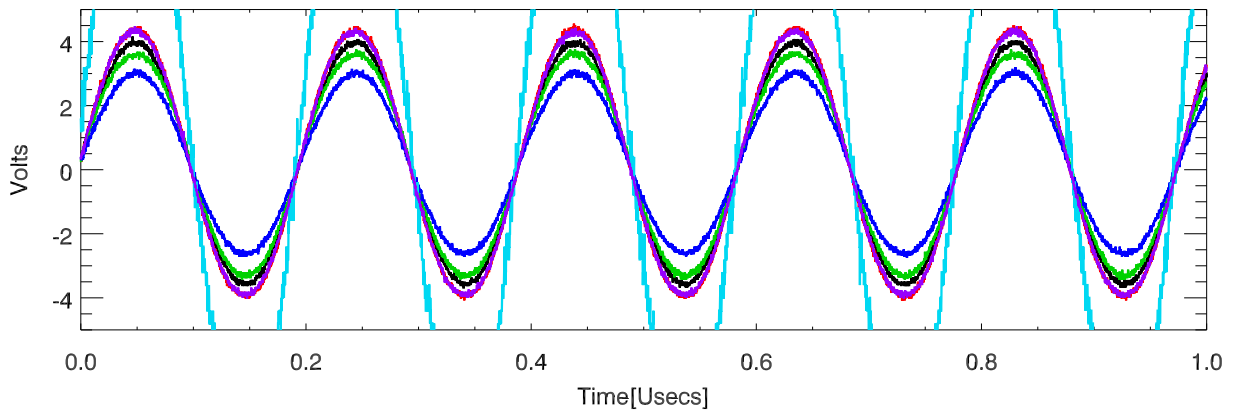
151102 overplot tube output ports. IPA Anode
