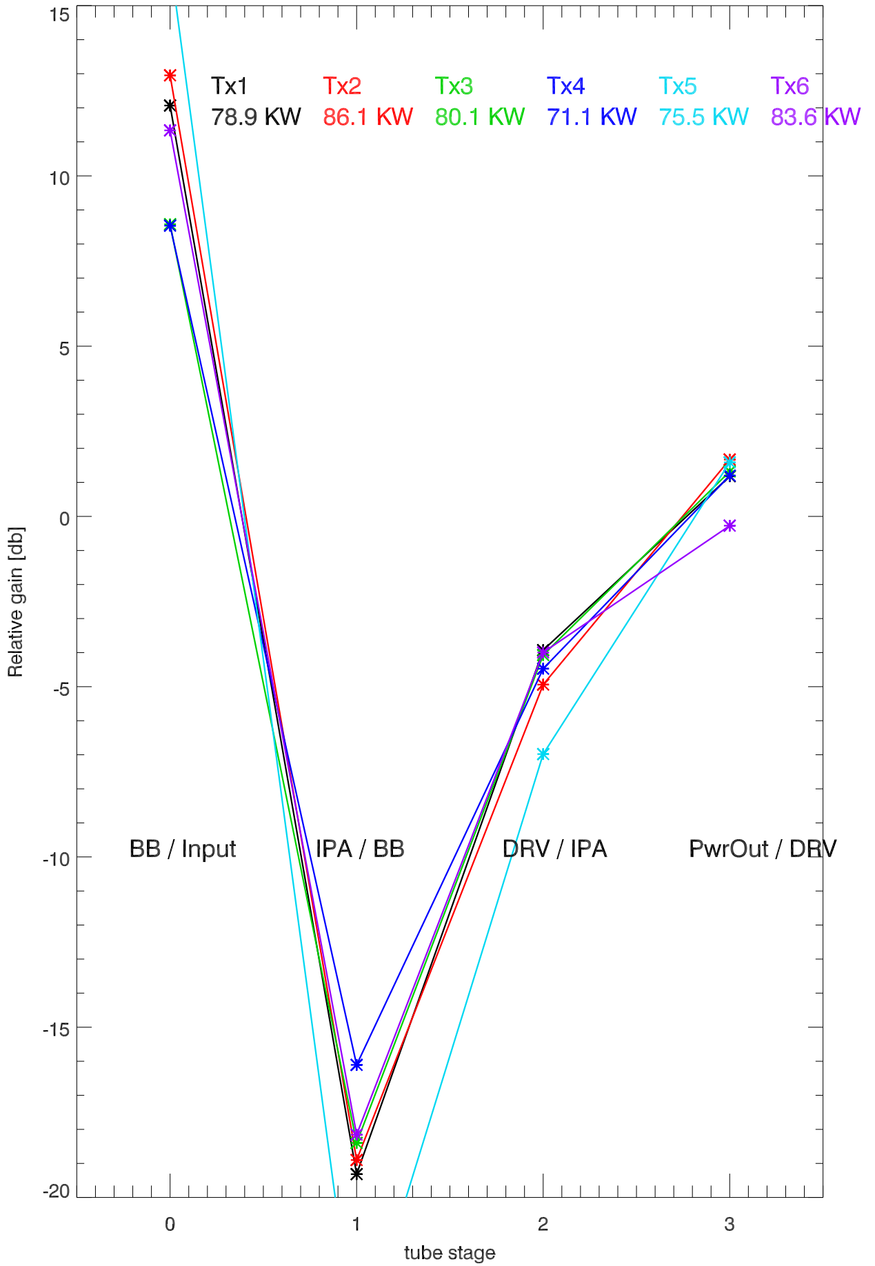
151102 relative gain of tube stages. ( P_{\text{w}}\text{Out}[n+1]/P_{\text{w}}\text{Out}[n] )
