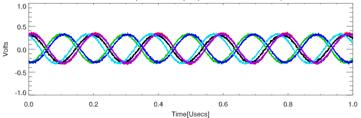
151102 overplot tube output ports. RF FwdPwr Output
